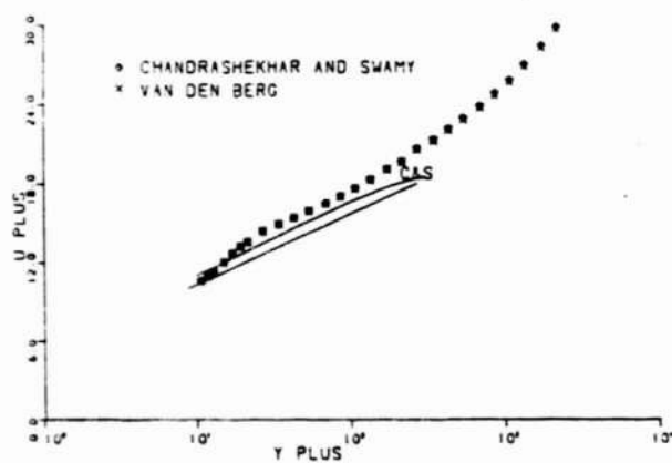
Fig. 6.4 Three-Dimensional Similarity Plots for C7
