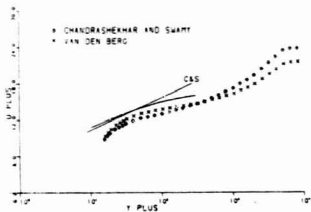
Fig. 6.18 Three-Dimensional Similarity Plots for E1
