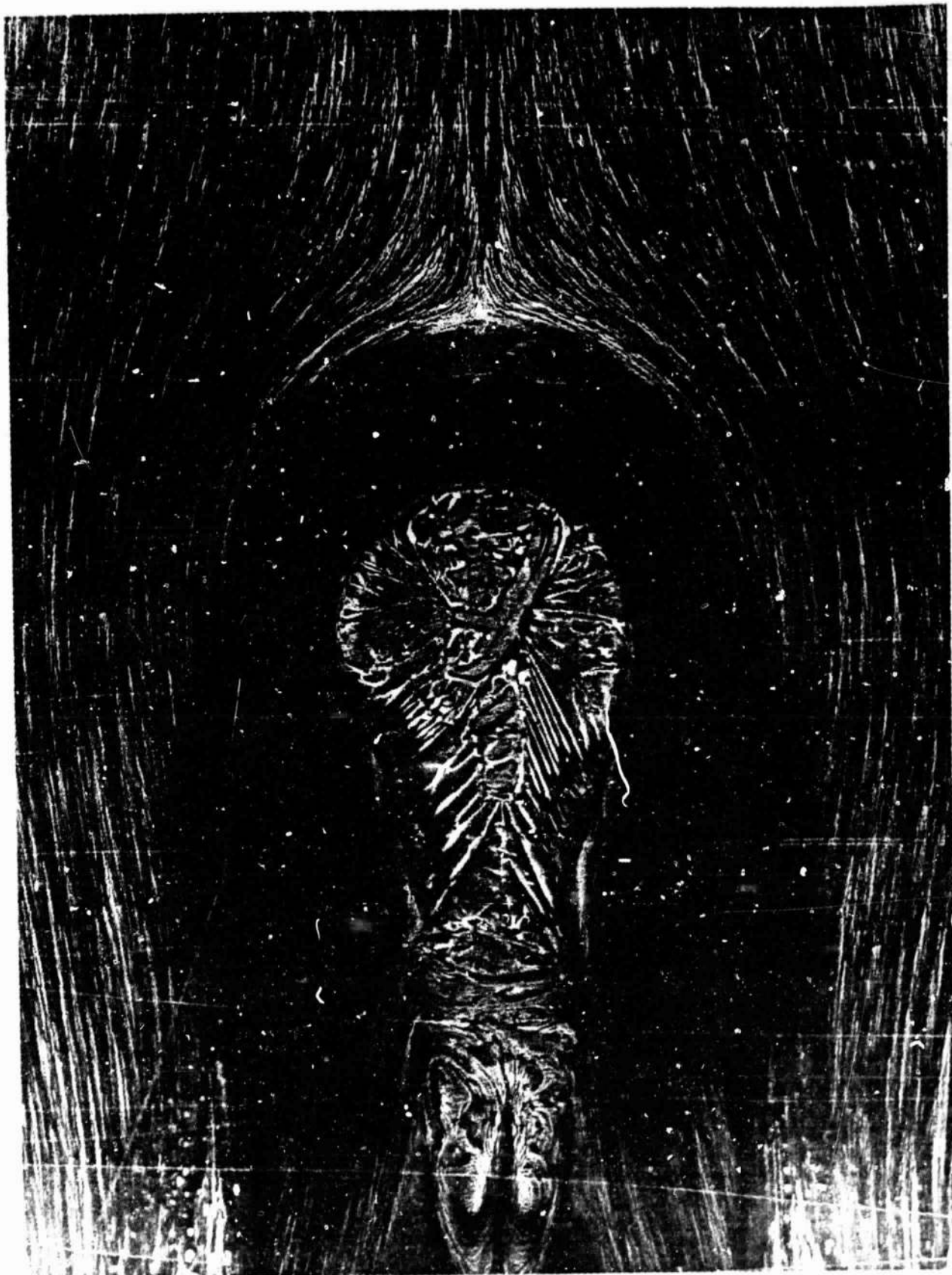
Fig. 5.15 Oil Streak Pattern
