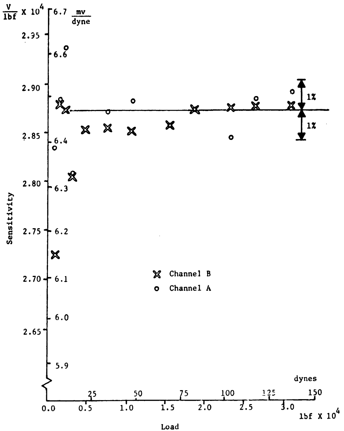
Fig. 3.8 Individual Load Sensitivities for the Omnidirectional Meter Calibration Curves
