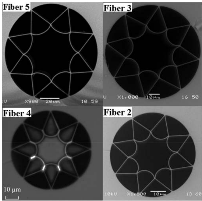
Fig. 7. SEM and optical microscope pictures of some NC-NCFs designed for similar transmission windows in Table I. SEM images of Fibers 5, 3 and 2, and an optical micrograph of Fiber 4 as labelled. Fibers 3 and 2 have lower attenuation than Fibers 4 and 5, respectively, despite being at approximately comparable wavelengths. The degradation of cladding structure, such as the slab-like fusion between capillaries (Fiber 4) and reduced boundary curvature (Fiber 5) may result in such higher losses. Fibers 3 and 2 were fabricated from the same preforms with fluorine-doped silica glass as the jacketing tube, and using a smaller draw-down ratio. Fibers 5 and 4 were fabricated using a pure silica glasses jacketing tube and a higher draw-down ratio.
