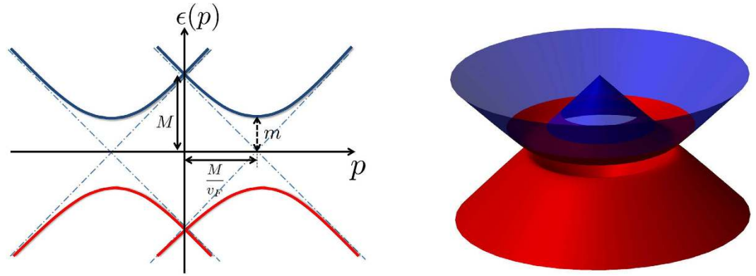
Figure 1. Left) The bandstructure of a Dirac ring system \pm\epsilon(p) given by Eq. 4, with asymptotic canonical velocity (slope) given by v_F\hat{k} . Right) 3D view of the same band structure, with the axis of rotation the energy axis and the plane of rotation the p_x, p_y plane. The occupied (red) band is separated from the partially occupied (blue) band by a mass gap 2m . They can be obtained by gapping out two intersecting Dirac cone with energy difference of 2M . A ring of filled states (red) at chemical potential \mu > m lies in the ring of minima on the valence (blue) band.
