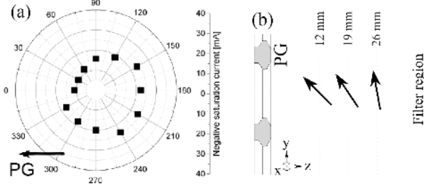
FIG. 7. (a) Polar distribution of negative saturation current in Cs seeded plasma and (b) flow direction of electron at z of 12, 19 and 26 mm.
