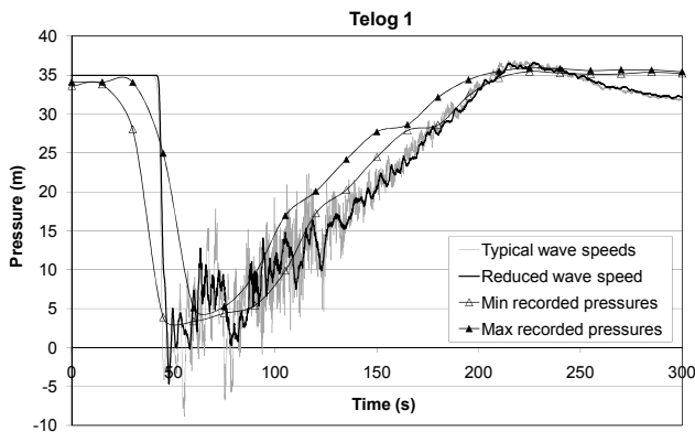
Figure 2. Comparison of pressures recorded at one distribution system site with pressures modelled with typical wave speeds and with a reduced wave velocity in cast-iron pipes (four pressure values per second were measured by the pressure recorders but only the minimum and maximum pressures over 15 s intervals were saved ( \Delta and \blacktriangle )).
