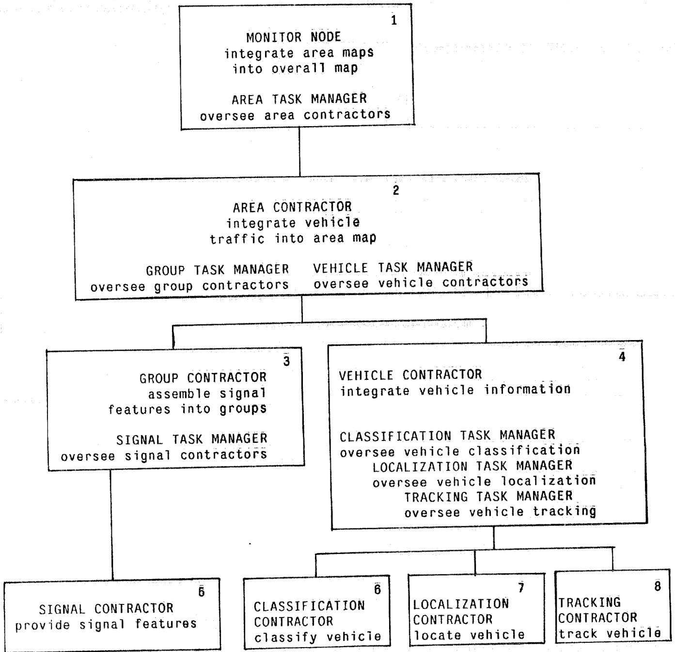
Fig. 15: Nodes and their roles.
