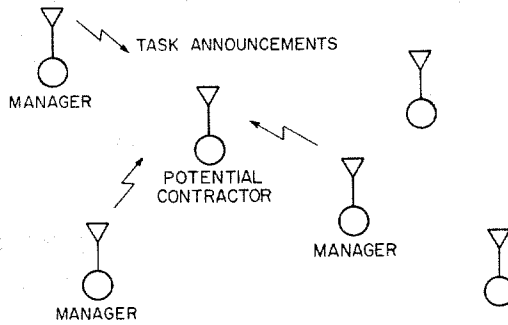
Fig. 5: Idle node listening to task announcements.
