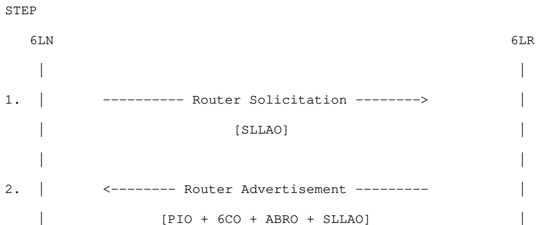
Figure 2: Basic Router Solicitation/Router Advertisement Exchange between a Node and a 6LR or 6LBR
