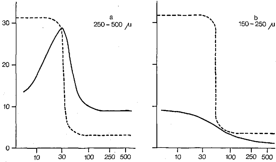
FIG. 5A. Horizontal migration of Ditylenchus dipsaci larvae through fractions of a sandy loam soil which are favourable (a) or too fine (b), at different suctions (after Wallace, 1958). —: mobility, ----: moisture content at different suctions. Abscissae: suction (cm water column, log. scale). Ordinates: moisture content (% by volume) as well as migration (% nematodes moving more than 3 cm in 5 hours).
