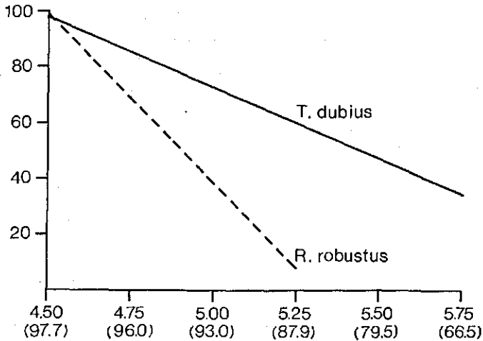
FIG. 20. Regression lines of percentages T. dubius and R. robustus females surviving 7 days of desiccation in vitro ( y ), on pF' values corresponding to the relative humidities applied ( x ) calculated from 6 replicates. r = regression coefficient.
