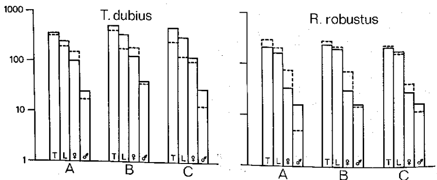
FIG. 12 A, B, C. Initial numbers (—) and numbers after 24 weeks (---) of populations of T. dubius and R. robustus in fallow sandy soil fluctuating between pF 0 and 4.2, indicated separately for total nematode numbers (T), larvae (L), females (♀) and males (♂), in three parallel experiments:
