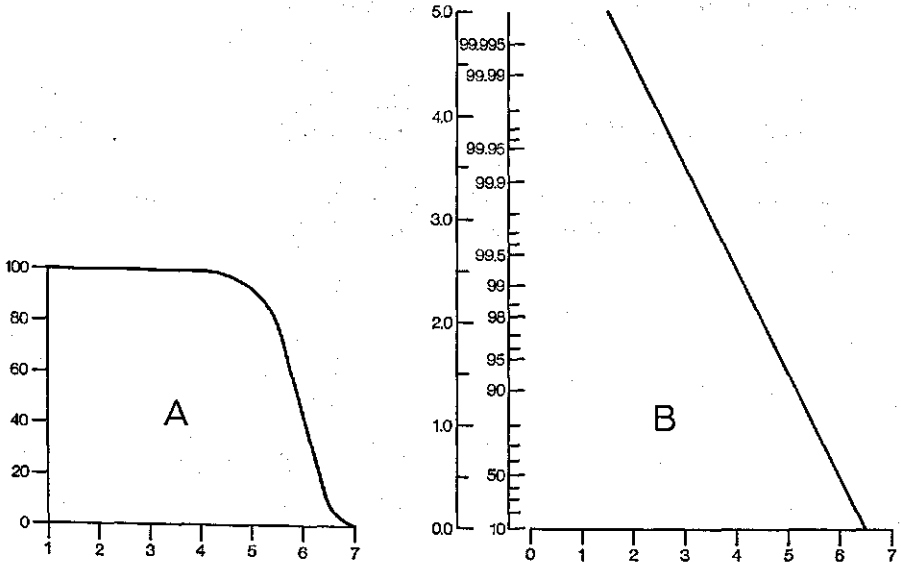
FIG. 4. Relation between pF' and relative humidity (r.h.) at 20°C (fig. A: Croney, Coleman and Bridge, 1952; fig. B: Stakman, 1968).
