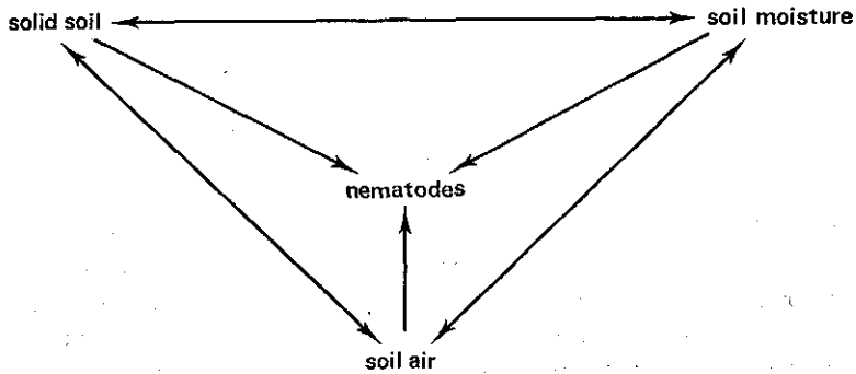
FIG. 1. Scheme of gross relations between the three major, interrelated soil phases and nematodes.
