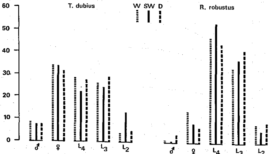
FIG. 15. Distribution of stages of development of populations of T. dubius and R. robustus extracted from dry soil by three different methods, indicated at W, SW and D (cf. fig. 14).
