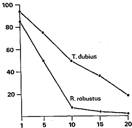
FIG. 21. Survival of T. dubius and R. robustus females after 1, 5, 10, 15 and 20 days exposure to 93.0% r.h.
