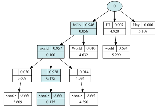
Figure 1: Search graph visualisation for DE→EN translation of "Hallo Welt!" with beam size 3.
