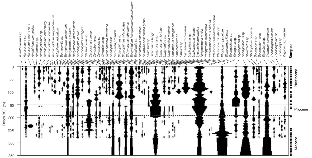
Figure. S5: Stratigraphic distribution of several radiolarian species and species group at Hole U1414A
