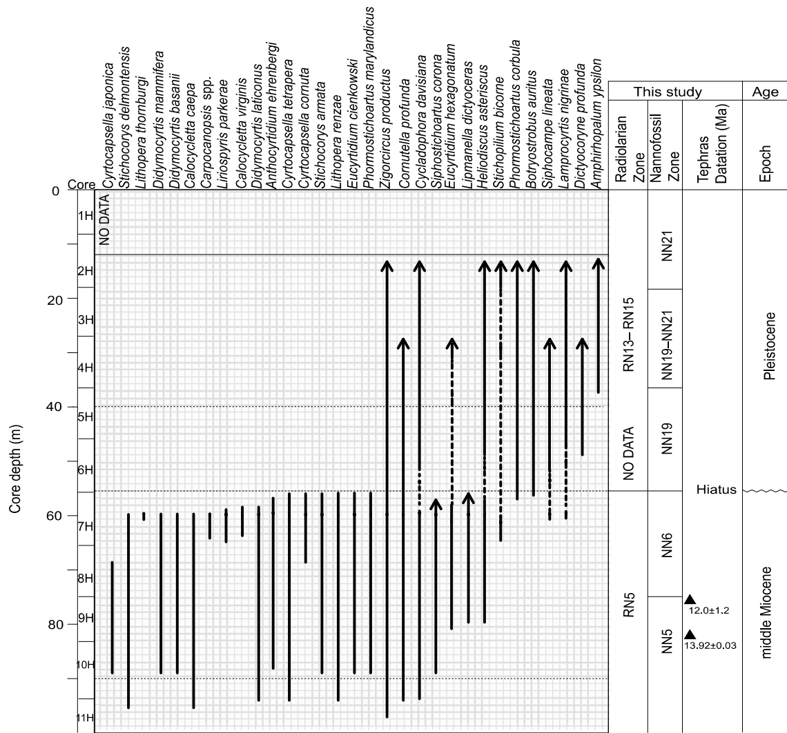
Figure S2. Diagram showing the distribution of common and biostratigraphically important radiolarian species in Hole U1381C. Calcareous nannofossil and tephra layer ages were used to correlate the radiolarian biozones. Solid lines with arrows: extant species. Dashed lines: species with known stratigraphic distribution but absent in our materials. The hiatus in this sequence is ~8 m.y. long.
