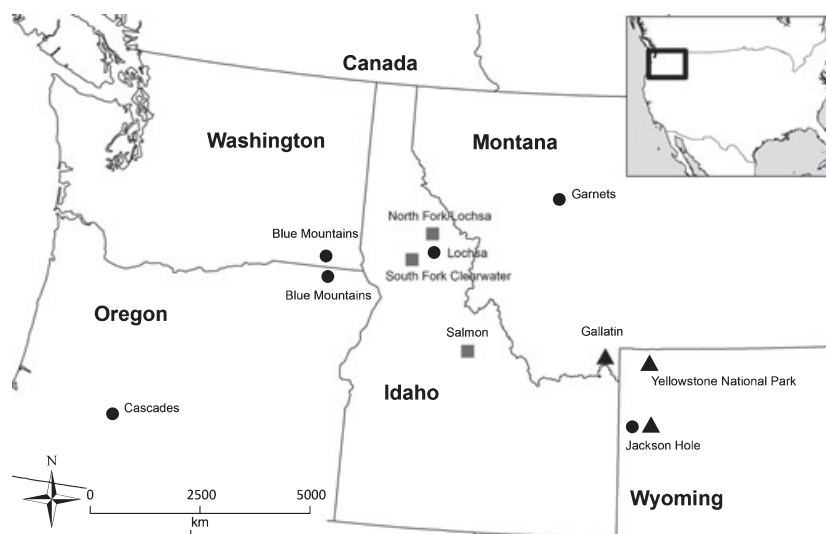
Fig. 1. Location of 12 study areas in the north-western USA, from 1973 to 2007. Black circles indicate study areas with three major predators (cougar, black bears and coyotes); grey squares indicate areas with three major predators prior to 2001 and four major predators (same predators as three-predator system plus wolves) after 2001; and black triangles indicate areas with five predators (same predators as the four-predator system plus grizzly bear). Note that two different studies occurred in Jackson Hole, WY between which additional predator species moved into the area.
