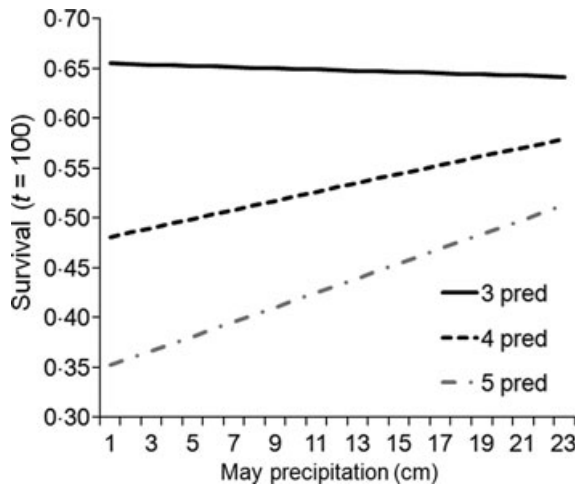
Fig. 3. Neonatal elk survival at day 100 as a function of May precipitation (cm) under different number of predator species across the north-western United States, 1973–2007.
