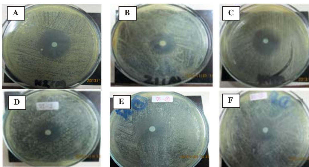
Figure 2. Results of disc diffusion test of non-induced liquid (NIL), prey-induced liquid (PIL), and chitin-induced liquid (CIL) to C. albicans and C. glabrata . Inhibition zone of NIL to C. albicans (A), PIL to C. albicans (B), CIL to C. albicans (C), NIL to C. glabrata (D), PIL to C. glabrata (E), CIL to C. glabrata (F)
