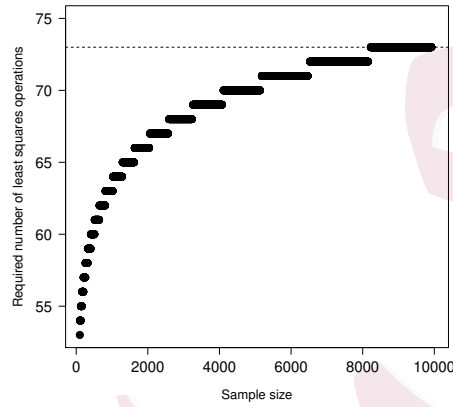
Figure 2: The total required number of least squares operations in (3.7).
