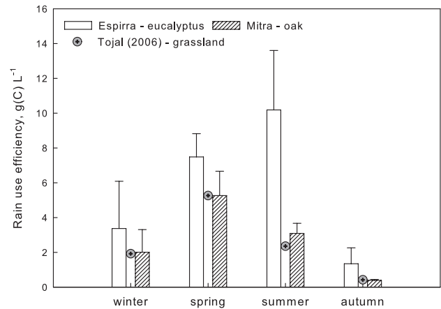
Fig. 7. Seasonal variation in GPP rain use efficiency (GPP/precipitation, \text{gCL}^{-1} ) in two experimental sites (Espirra – eucalyptus plantation and Mitra – oak woodland) during the experimental period (4 years – 2003–2006 – averages with standard error). The 2006 value for the Tojal grassland is also shown.
