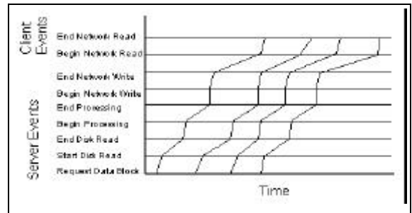
Figure 3: NetLogger lifelines
