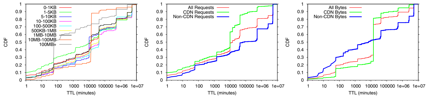
Figure 6: TTL of Cache Directives for HTTP Requests Figure 7: TTL of Cache Directives for requests Figure 8: TTL of Cache Directives for requests Weighted by Bytes
