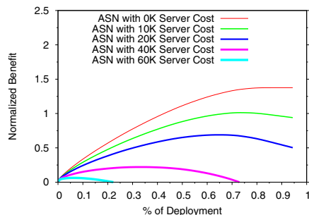
Figure 14: Benefits for Different Server Costs (fixed $4 Transit, $4 Backbone, 400 Mbps, 4TB)
