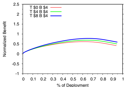
Figure 12: Benefits for Different Transit Costs
