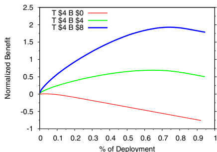
Figure 13: Benefits for Different Backbone Costs
