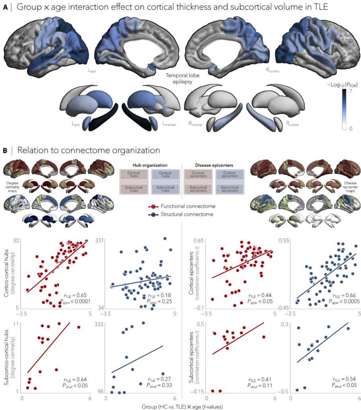
Fig. 4. Negative effects of age on cortical thickness and subcortical volume in TLE. (A) Significant age-related differences on gray matter atrophy between individuals with TLE and healthy controls for all cortical and subcortical regions. Patients with TLE showed a negative effect of age on cortical thickness in bilateral temporo-parietal ( P_{FDR} < 0.005 ) and sensorimotor ( P_{FDR} < 0.01 ) cortices and on subcortical volume in ipsilateral hippocampus ( P_{FDR} < 5 \times 10^{-7} ) and bilateral thalamus ( P_{FDR} < 0.05 ). Negative \log_{10} -transformed FDR-corrected P values are shown. (B) Schematic of the figure layout is provided in the middle. Scatterplots depict relationships between the age-related effects and functional (red) and structural (blue) maps of degree centrality (left) and disease epicenter (right). Significant associations were observed between age-related effects and every hub and epicenter measures, with the exception of structural subcortical degree centrality, suggesting a role of connectome organization on age-related effects in TLE.
