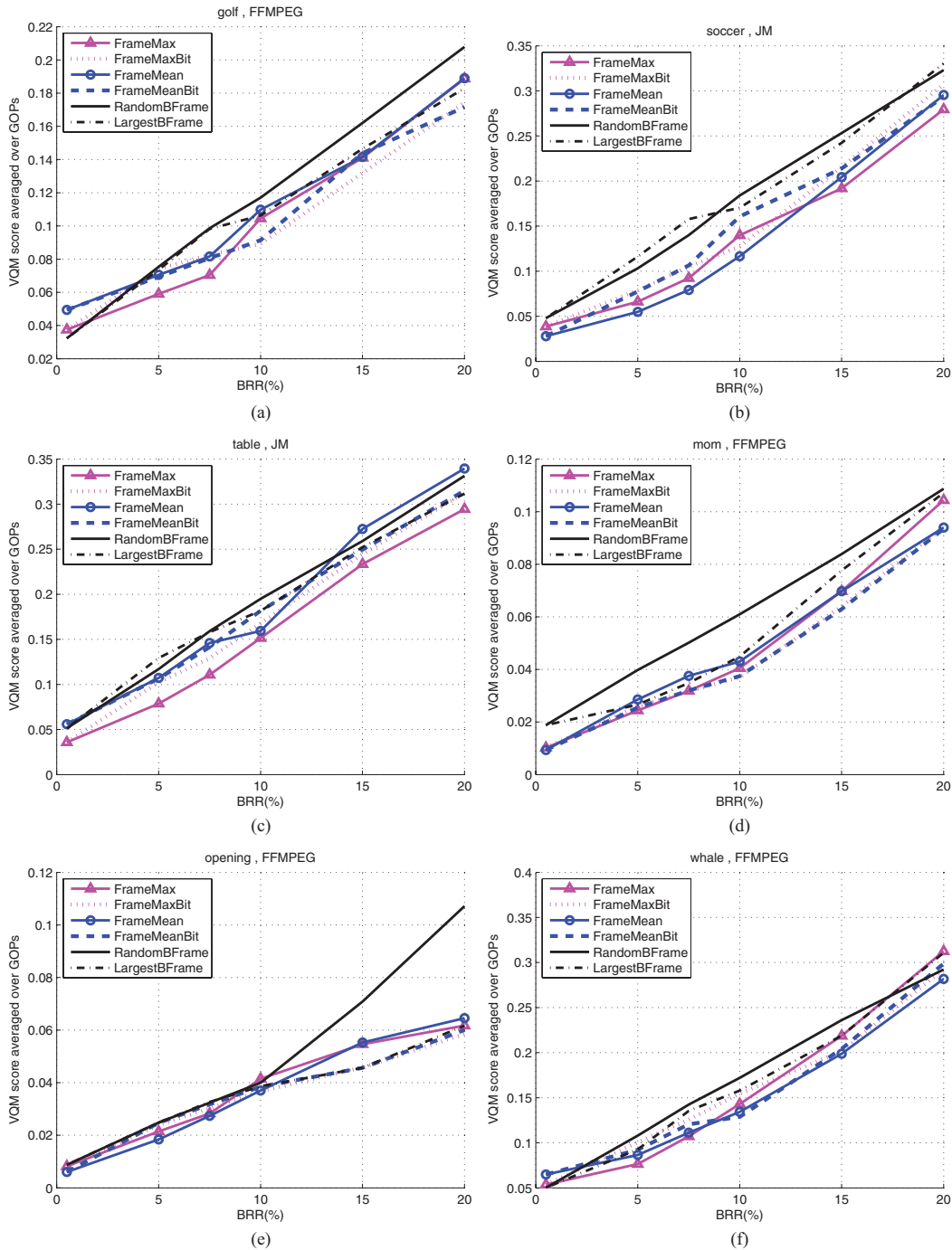
Fig. 10. Average VQM score over GOPs versus BRR for the six packet dropping policies for (a) FFMPEG for Golf , (b) JM for Soccer , (c) JM for Table tennis , (d) FFMPEG for Mother Daughter , (e) FFMPEG for Opening , and (f) FFMPEG for Whale . Lower VQM scores correspond to higher quality.
