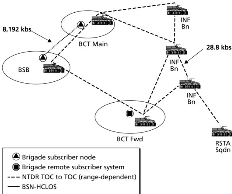
Figure 4.4 SBCT TOC-to-TOC C2 Node Subnet
