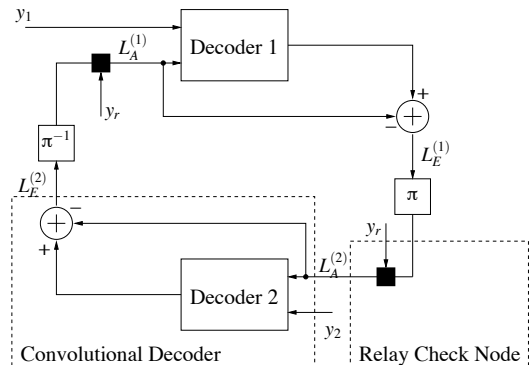
Fig. 3. Iterative decoding
