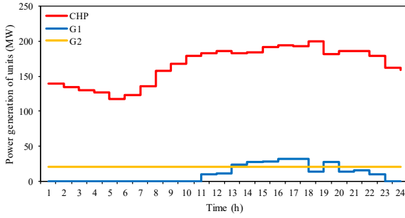
Fig. 5. Power generation scheduling of the plants in case 1
