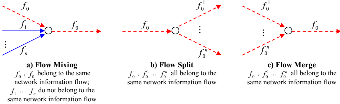
Figure 2. Inter-flow transformations
