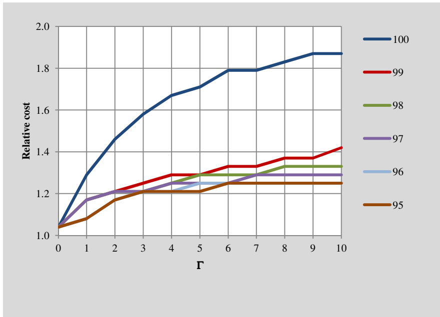
Figure 3: Price of robustness (relative to \Gamma = 0 ) for robust network design on the basis of historical data for the pan-European research backbone network GÉANT with observed means as nominal values and subject to different quintiles for the peak demand values (nominal + deviation).
