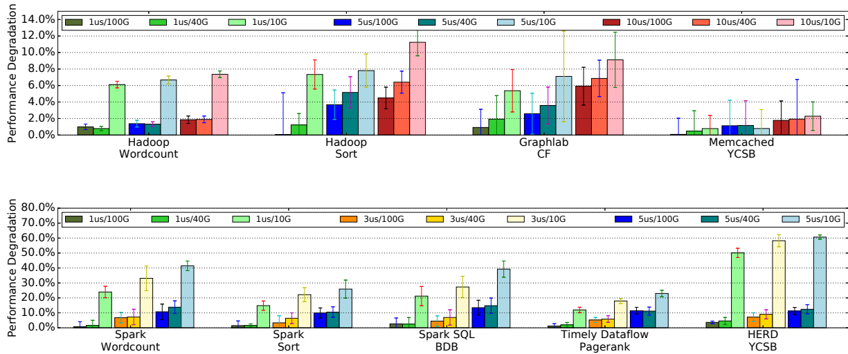
Figure 2: Comparison of application-level performance in disaggregated datacenters with respect to existing server-centric architectures for different latency/bandwidth configurations and 25% local memory on CPU blades — Class A apps (top) and Class B apps (bottom). To maintain application-level performance within reasonable performance bounds ( \sim 5\% on an average), Class A apps require 5\mu\text{s} end-to-end latency and 40Gbps bandwidth, and Class B apps require 3\mu\text{s} end-to-end latency and 40–100Gbps bandwidth. See §3.2 for detailed discussion.
