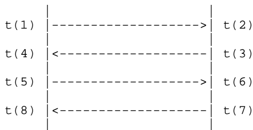
Figure 3.1. Calculating Delay and Offset
