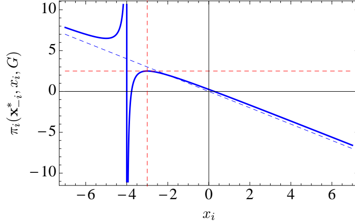
FIGURE I. THE PAYOFF FUNCTION \pi_i(\mathbf{x}_{-i}^*, x_i, G) FROM EQUATION (A10) FOR DIFFERENT VALUES OF x_i . THE HORIZONTAL RED DASHED LINE INDICATES \pi_i^* , THE RED VERTICAL DASHED LINE INDICATES x_i^* , WHILE THE BLUE VERTICAL SOLID LINE INDICATES THE POINT OF DISCONTINUITY, -B_i^{\beta,\gamma}(G) . IF x_i IS LARGER THAN THE DISCONTINUITY AT -B_i^{\beta,\gamma}(G) THEN WE HAVE THAT \pi_i(\mathbf{x}_{-i}^*, x_i, G) < \pi_i(\mathbf{x}^*, G) . THE BLUE DASHED LINE INDICATES THE ASYMPTOTE WITH SLOPE -1 .
