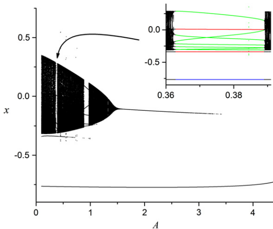
Fig. 6. Bifurcation diagram showing the asymptotic behavior of the macroscopic mean field, obtained using Eq. (18), versus the amplitude A of the excitability modulation (defined in Eq. (4)). The macroscopic mean field z was sampled stroboscopically with period \tau before x = \text{Re}(z) was plotted, and many initial conditions were used for each value of A in order to identify coexisting attractors. Other parameters were \eta_0 = 10.75 , k = -9 , \Delta = 0.5 , and \tau = 1 . The structure with dark bands on the left reflects quasiperiodic behavior. Periodic orbits appear as sets of lines. The inset is a magnification showing the thin periodic window near A = 0.38 . The three coexisting periodic orbits within this window are color coded according to the color scheme used in Fig. 11. (For interpretation of the references to colour in this figure legend, the reader is referred to the web version of this article.)
