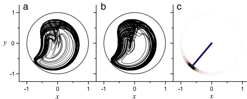
Fig. 8. (a) A predicted chaotic attractor, obtained using the reduced mean field equation (Eq. (18)) with \eta_0 = 10.75 , k = -9 , \Delta = 0.5 , A = 4.8 , and \tau = 1 . (b) The asymptotic trajectory of the macroscopic mean field, obtained using a discrete network of 10,000 neurons at the same parameters. (c) A snapshot showing the microstate at a particular time. The blue line indicates the instantaneous macroscopic mean field variable z , and the red dots show the distribution of phases, with darker regions denoting higher density. (For interpretation of the references to colour in this figure legend, the reader is referred to the web version of this article.)
