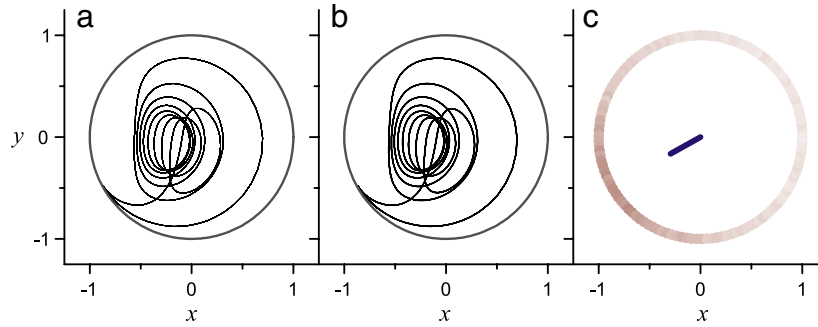
Fig. 10. The period- \tau_9 orbit with winding number 9 created by the sequence of period-adding bifurcations shown in Fig. 9(c). (a) The predicted orbit obtained using the reduced mean field equation (Eq. (18)) with \eta_0 = 10.75 , k = -9 , \Delta = 0.5 , A = 4.8 , and \tau = 25 . (b) The asymptotic trajectory of the macroscopic mean field, obtained using a discrete network of 10,000 neurons at the same parameters. (c) A snapshot showing the microstate at a particular time. The blue line indicates the instantaneous macroscopic mean field variable z , and the red dots show the distribution of phases, with darker regions denoting higher density. (For interpretation of the references to colour in this figure legend, the reader is referred to the web version of this article.)
