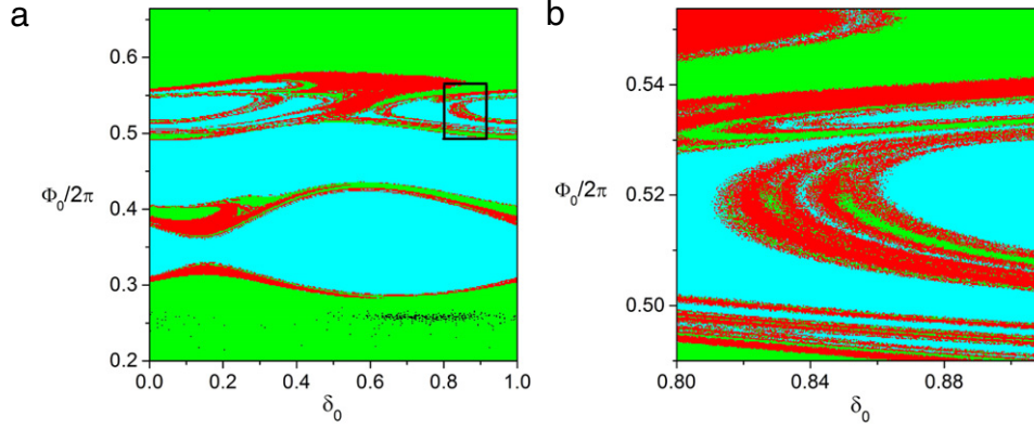
Fig. 12. Basins of attraction for the attractors shown in Fig. 11, obtained using a discrete network of 10,000 neurons. Panel (b) is a magnification of the region marked by the black rectangle in panel (a). Initial conditions for the discrete network consist of a point (\delta_0, \Phi) on this graph, with x_0 = 0.45 and y_0 = -0.3 .
