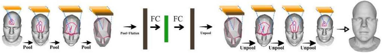
Figure 1: Illustration of our Neural3DMM architecture
