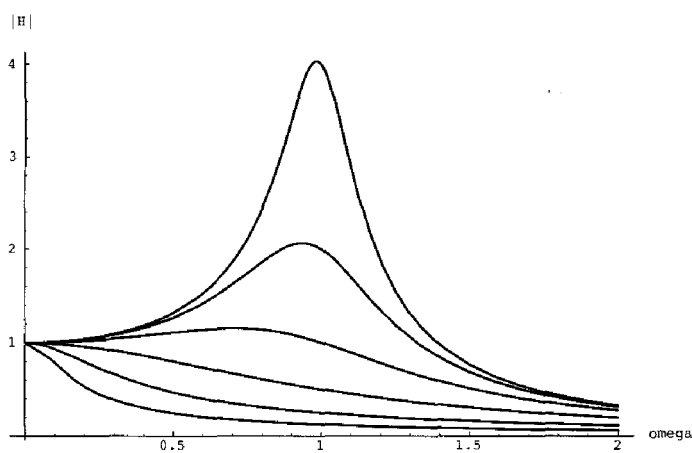
Figure 2.8: |H(\omega)| for \tau_{2,ik} = 1 and Q \in \left\{ \frac{1}{8}, \frac{1}{4}, \frac{1}{2}, 1, 2, 4 \right\} .
