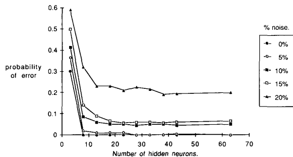
Fig. 3. Network architecture as assessed by crossvalidation for classification of random patterns. The figure shows performance versus number of hidden neurons using test sets with 0, 5, 10, 15, and 20% probability of bit inversion in the input.
