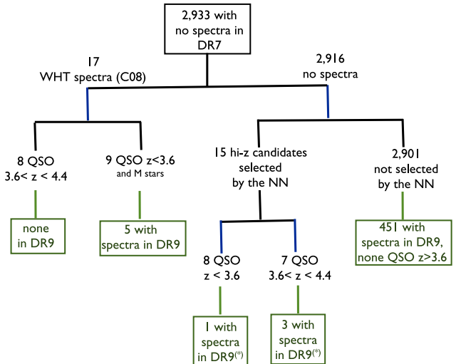
Figure 5. Schematic overview of a check of the efficiency of our selection via comparison with DR9 spectroscopic information. See Section 4.2. The 2916 objects (Section 3.2) without spectra in DR7, or in the literature, were classified by our NN, with 15 being selected by the NN as high-redshift candidates. (*) = targets from BOSS (Baryon Oscillations Spectroscopic Survey).
