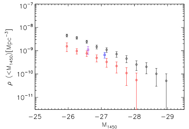
Figure 13. Cumulative LFs at z = 3.8 (black circles) and z = 4.2 (red circles). Squares represent densities derived by Vigotti et al. (2003, blue square) and Carballo et al. (2006, purple square) at redshifts z \sim 4.1 and 4 , respectively.
