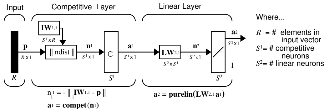
LVQ Architecture
