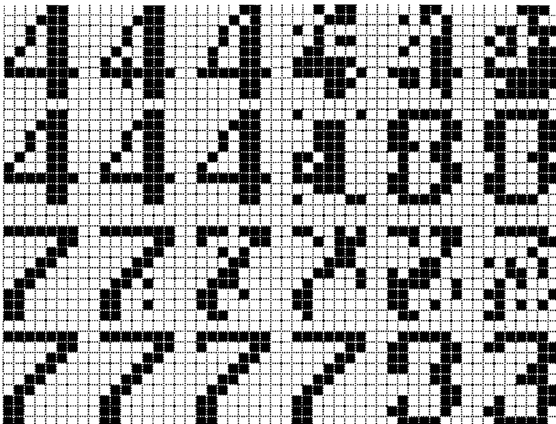
FIG. 6b. Performance of Hopfield network on error-corrupted input.
