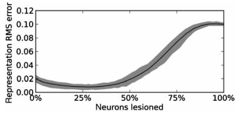
Figure 7. Representation accuracy as neurons are lesioned in order of locality. 5000 neurons are used to represent a 100-dimensional vector x . Neurons are destroyed in order of sensitivity to the particular x value represented, starting with the most local. Grey area is minimum/maximum error over 50 trials. The most local 50% of neurons can be completely destroyed before we see significant decreases in representation accuracy.
