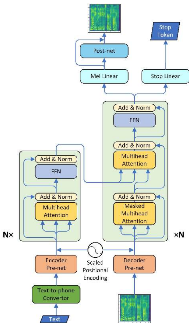
Figure 3: System architecture of our model.
