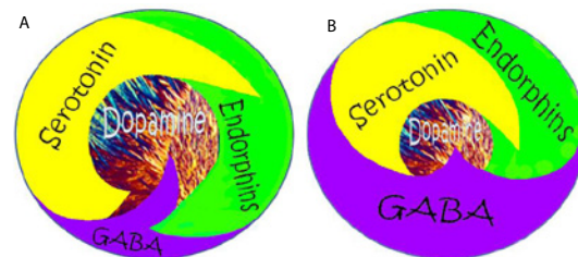
Figure 2: Brain reward cascade (normal and hypodopaminergic state).
