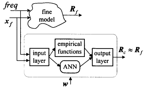
Fig. 4. KBNN neuromodeling concept [7].
