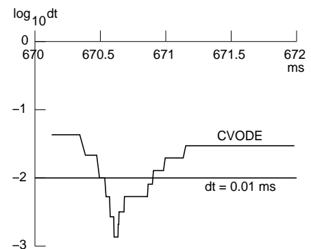
B. The \Delta t used by CVODE was > 0.01 ms throughout the entire simulation except for brief intervals that extended from just before the threshold of each spike until shortly after its peak.
