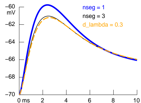
B. Time course of V_{soma} computed using spatial grids with one or three nodes per branch (thick blue and thin black traces for nseg = 1 and 3, respectively) or specified by the d\_lambda = 0.3 criterion (dashed orange trace).
