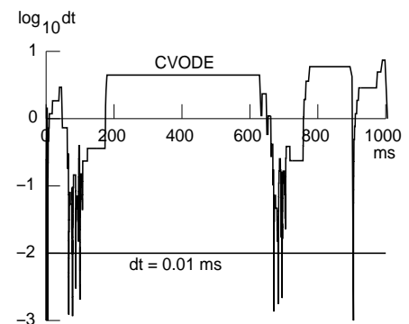
B. The \Delta t used by CVODE varied over a wide range, dropping below 0.01 ms transiently during each action potential, and at three instants: the very beginning of the simulation ( t = 0 ms), and at the abrupt start and end of the injected current pulse (5 ms and 905 ms). However for most of the simulation \Delta t was much larger than 0.01 ms. The order of integration ranged from 2 to 5, with most steps using second or third order integration.
