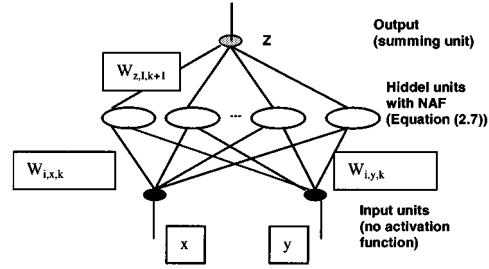
Fig. 2. 2-D NAHONN structure.
