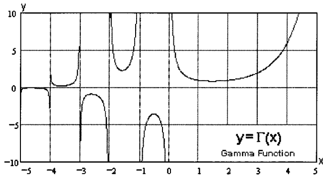
Fig. 8. Gamma-function.
