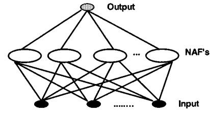
Fig. 5. NANONN with one output.
