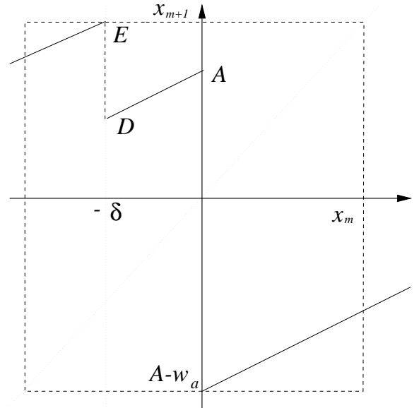
FIG. 11. Graph of the piecewise linear map \mathcal{F} . Dashed rectangle indicates region of convergence.
