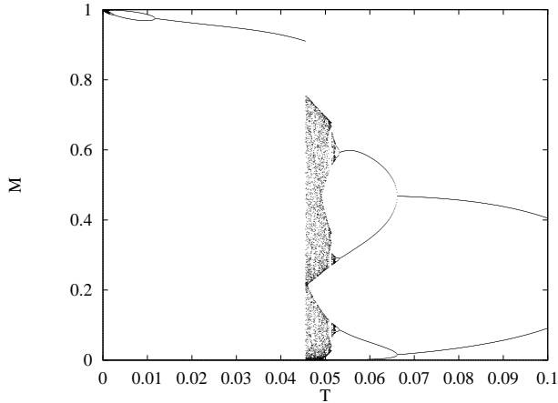
FIG. 10. Global hysteresis in mean activity: Temperature decreasing. w_a = 1.0 , w_b = 0.4 , \delta = 0.5 , \gamma = 0.75 , I = 0.2 .
