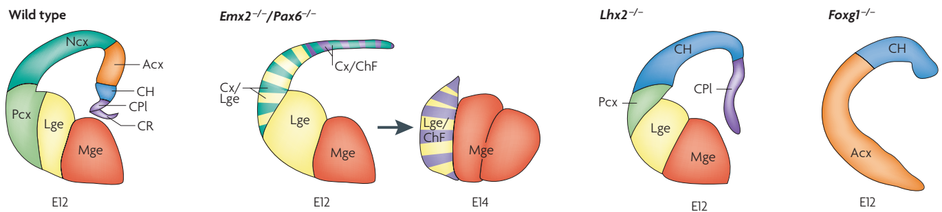
Figure 2 | Emx2 , Pax6 , Lhx2 and Foxg1 have crucial roles in the specification of neocortical progenitors. Loss of both empty spiracle homologue 2 ( Emx2 ) and paired box 6 ( Pax6 ) results in ventralization of cortical progenitors and the loss of the neocortical domain (Ncx), archicortex (Acx), cortical hem (CH) and choroid plexus (CPI) by embryonic day (E) 14 (REFS 67, 132). Loss of LIM homeobox 2 ( Lhx2 ) results in the expansion of the CPI and CH medial domains and the elimination of progenitors with neocortical identity 60–62 . Similarly, loss of forkhead box G1 ( Foxg1 ) causes agenesis of the basal ganglia, elimination of neocortical progenitor domains and expansion of the CH and the Acx 63,64 . CR, choroidal roof; ChF, choroid field (choroid plexus and choroidal roof); Cx, cortex; Lge, lateral ganglionic eminence; Mge, medial ganglionic eminence; Pcx, paleocortex. Modified, with permission, from REF. 133 (2003) Oxford Univ. Press.
