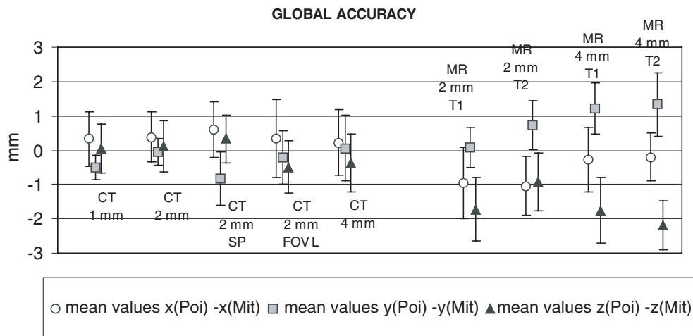
Figure 8. Mean values \overline{\Delta x^{P-M}}, \overline{\Delta y^{P-M}}, \overline{\Delta z^{P-M}}; \sigma_x^{P-M}, \sigma_y^{P-M}, \sigma_z^{P-M} are shown as error bars. Mean values of procedures based on MR imaging show meaningful deviations from the expected 0 value, especially in the z direction.
