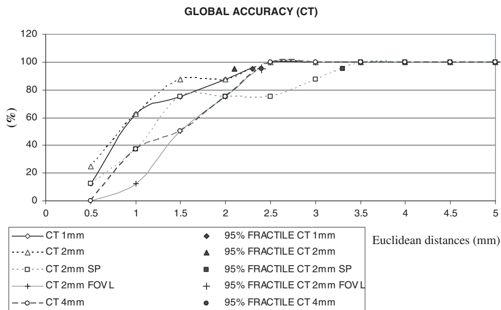
Figure 10. Cumulative distributions of the Euclidean distances \Delta r^{P-M} for procedures based on CT images. The 95% fractile of each distribution is also plotted. Different behaviour between CT 2 mm FOV L and CT 2 mm SP series can be observed. The 95% fractile of the CT 2 mm FOV L series coincides with that of the CT 4 mm series.
