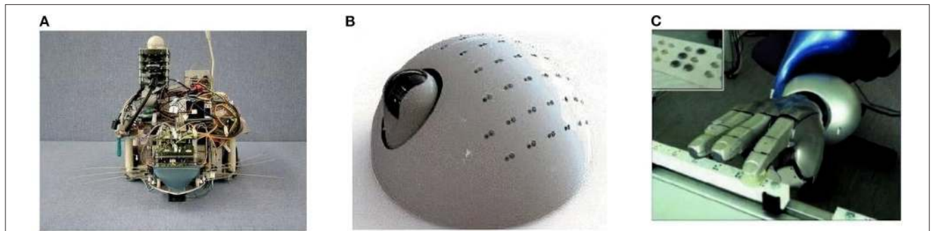
FIGURE 2 | Examples of neurorobots using tactile perception of the environment to generate explainable behavior. (A) The Whiskerbot, a robot that emulates rodent whisker sensory system for navigation (Pearson et al., 2007). (B) CARL-SJR, an anteater robot that interacts with human users by flashing multi-colored LEDs in response to rubbing gestures on its back (Bucci et al., 2014). (C) A neurobotic hand for fine tactile sensing, such as reading Braille characters (Bologna et al., 2013).
