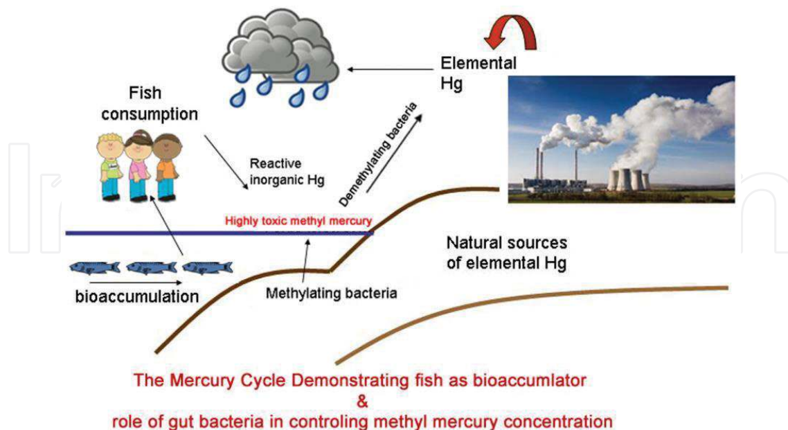
Figure 1. Role of fish in the bioaccumulation of mercury (Hg) and role of methylating and demethylating bacteria in the control of methyl mercury (MeHg) concentration as environmental neurotoxin related to autism.
