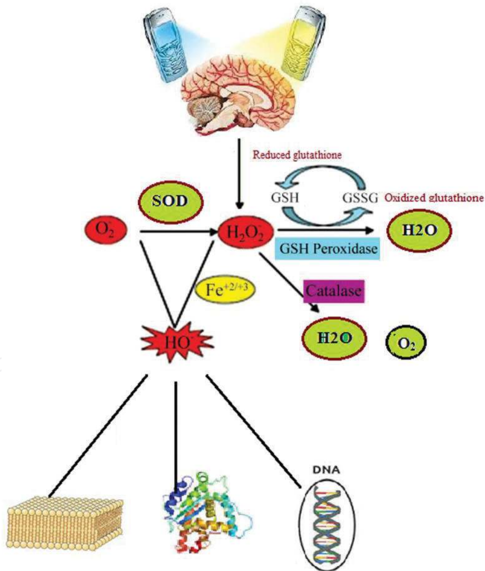
Figure 5. Role of cell phone radiation in the etiology of autism through oxidative stress as a major etiological mechanism.
