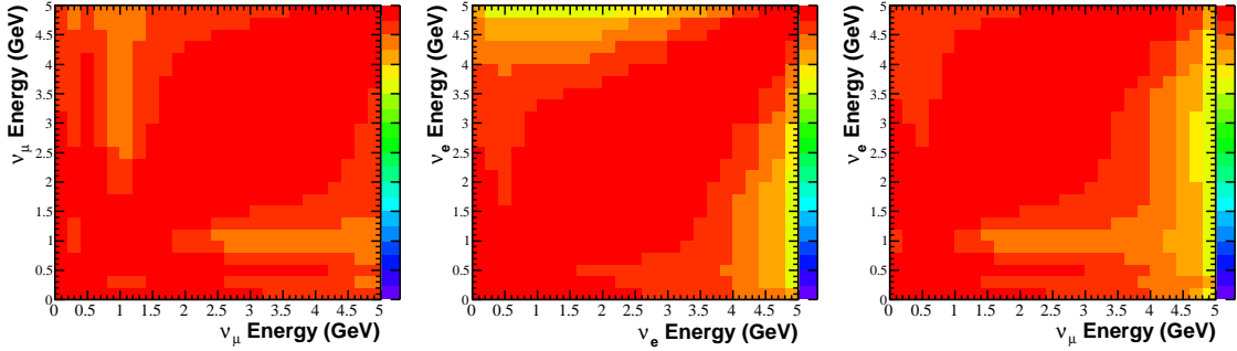
FIG. 35: Left: Correlation matrix for variations in the \pi^+ \rightarrow \nu_\mu flux due to uncertainties in \pi^+ production in p-Be interactions with the horn in neutrino mode. Center/Right: Same for variations in the \pi^+ \rightarrow \mu^+ \rightarrow \nu_e flux (center) and correlations between the \pi^+ \rightarrow \nu_\mu flux and the \pi^+ \rightarrow \mu^+ \rightarrow \nu_e flux (right). The color scale on each plot ranges from 0 to 1.
