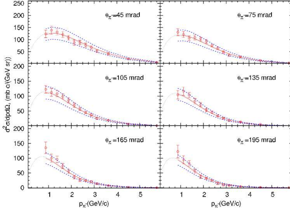
FIG. 22: Comparison of HARP \pi^- production cross section data [52] (red circles) versus p_\pi in bins of \theta_\pi from 8.89 GeV/c p-Be interactions and best-fit SW model (red line). The dashed blue lines represent the uncertainty band resulting from varying the parameters within their correlated uncertainties, as described in the text.
