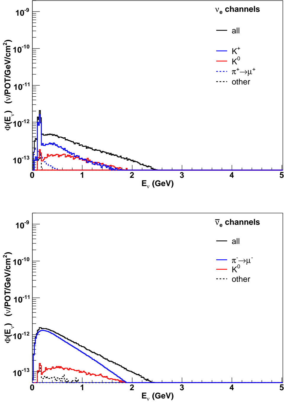
FIG. 32: Predicted \nu_e (top) and \bar{\nu}_e (bottom) fluxes at the MiniBooNE detector by parent meson species with horn in anti-neutrino mode. The black line is the total predicted flux, while all the subcomponents apart from the dashed black are from nucleon-induced meson production. The dashed black histogram includes all other contributions, primarily from meson decay chains initiated by meson-nucleus interactions.
