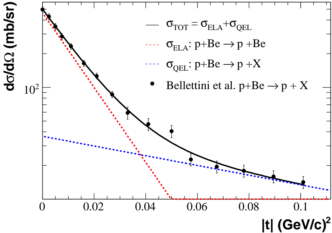
FIG. 39: Observed q^2 distribution from Bellettini et al. [64] for 20 GeV/c p-Be scattering. The black line represents the fit to two exponential distributions with the dashed red and blue lines showing the elastic and quasi-elastic contributions, respectively.
