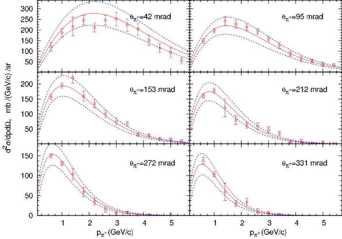
FIG. 21: Comparison of E910 \pi^+ production cross section data [44] (red circles) versus p_\pi in bins of \theta_\pi from 12.3 GeV/c p-Be interactions and best-fit SW model (red line). The dashed blue lines represent the uncertainty band resulting from varying the parameters within their correlated uncertainties, as described in the text.
