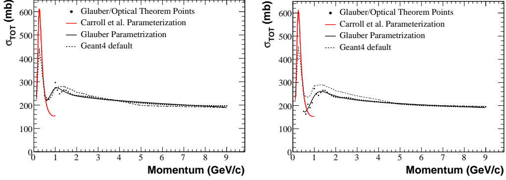
FIG. 12: Total hadronic cross sections for \pi^\pm -Be calculated using the Glauber model (black points) for \pi^+ (left) and \pi^- (right). The Breit-Wigner parametrization based on the Carroll data [37] on the \Delta(1232) resonance is shown as a red line, while the parametrization of the Glauber model points is shown as a solid black line. The Geant4 default model is shown as a dashed black line.
