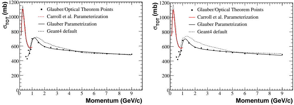
FIG. 13: Total hadronic cross sections for \pi^\pm -Al calculated using the Glauber model (black points) for \pi^+ (left) and \pi^- (right). The Breit-Wigner parametrization based on the Carroll data [37] on the \Delta(1232) resonance is shown as a red line, while the parametrization of the Glauber model points is shown as a solid black line. The Geant4 default model is shown as a dashed black line.
