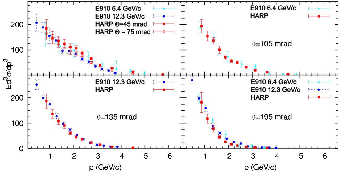
FIG. 26: Invariant pion production cross section from HARP and E910 versus p_\pi in bins of \theta_\pi . The E910 measurements are rescaled to p_B = 8.89 \text{ GeV}/c .
