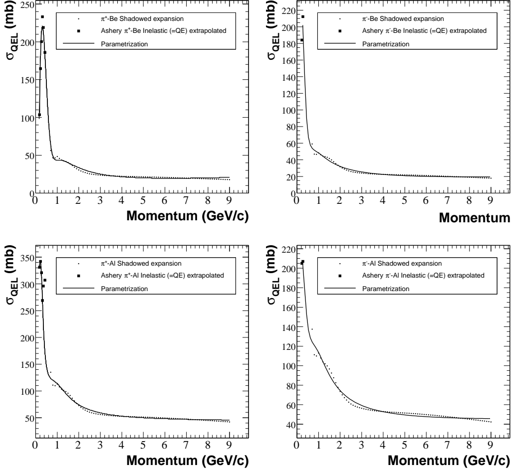
FIG. 17: Quasi-elastic cross sections for \pi^+ -Be (top left), \pi^- -Be (top right), \pi^+ -Al (bottom left) and \pi^- -Al (bottom right) as measured in References [40] (black squares) and calculated using the shadowed scattering model (black circles). The solid black lines are the parametrizations used in the flux prediction.
