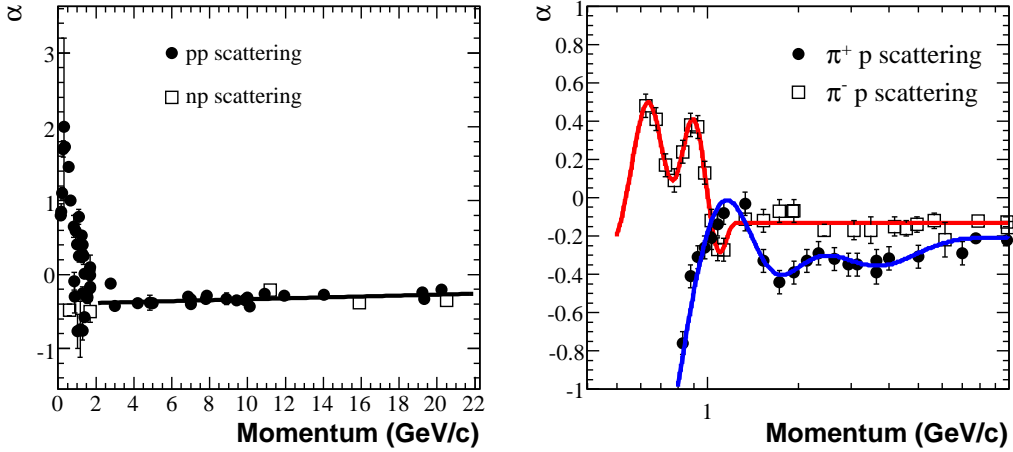
FIG. 8: Measured values of \alpha the real-to-imaginary ratio of the forward scattering amplitude for p - p and n - p scattering (left) and \pi^+ - p and \pi^- - p scattering (right) with parametrizations. The parametrizations used in the Glauber model calculation are shown.
