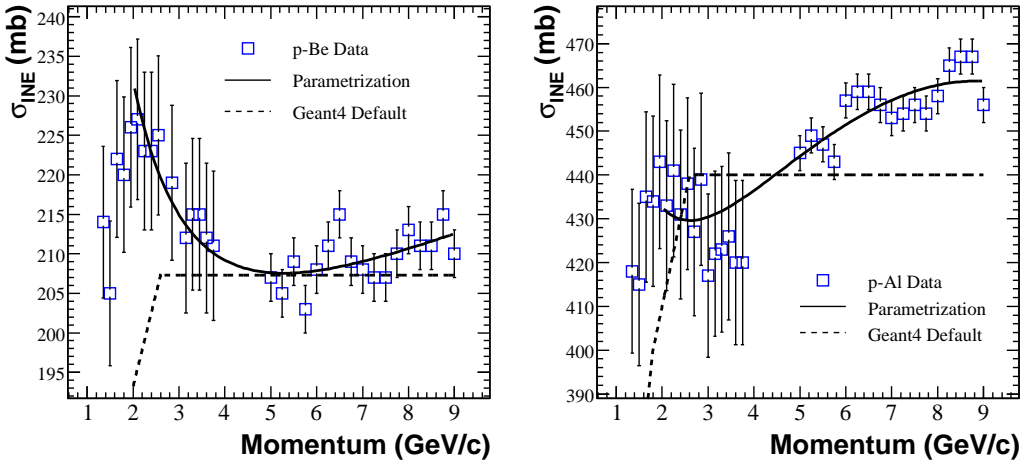
FIG. 14: p-Be (left) and p-Al (right) inelastic cross sections measured from Gachurin et al. [38] (1 – 4 GeV/c) and Bobchenko et al. [39] (5 – 9 GeV/c). The solid black line is the parametrization used in the flux prediction, while the dashed line shows the Geant4 default parametrization.
