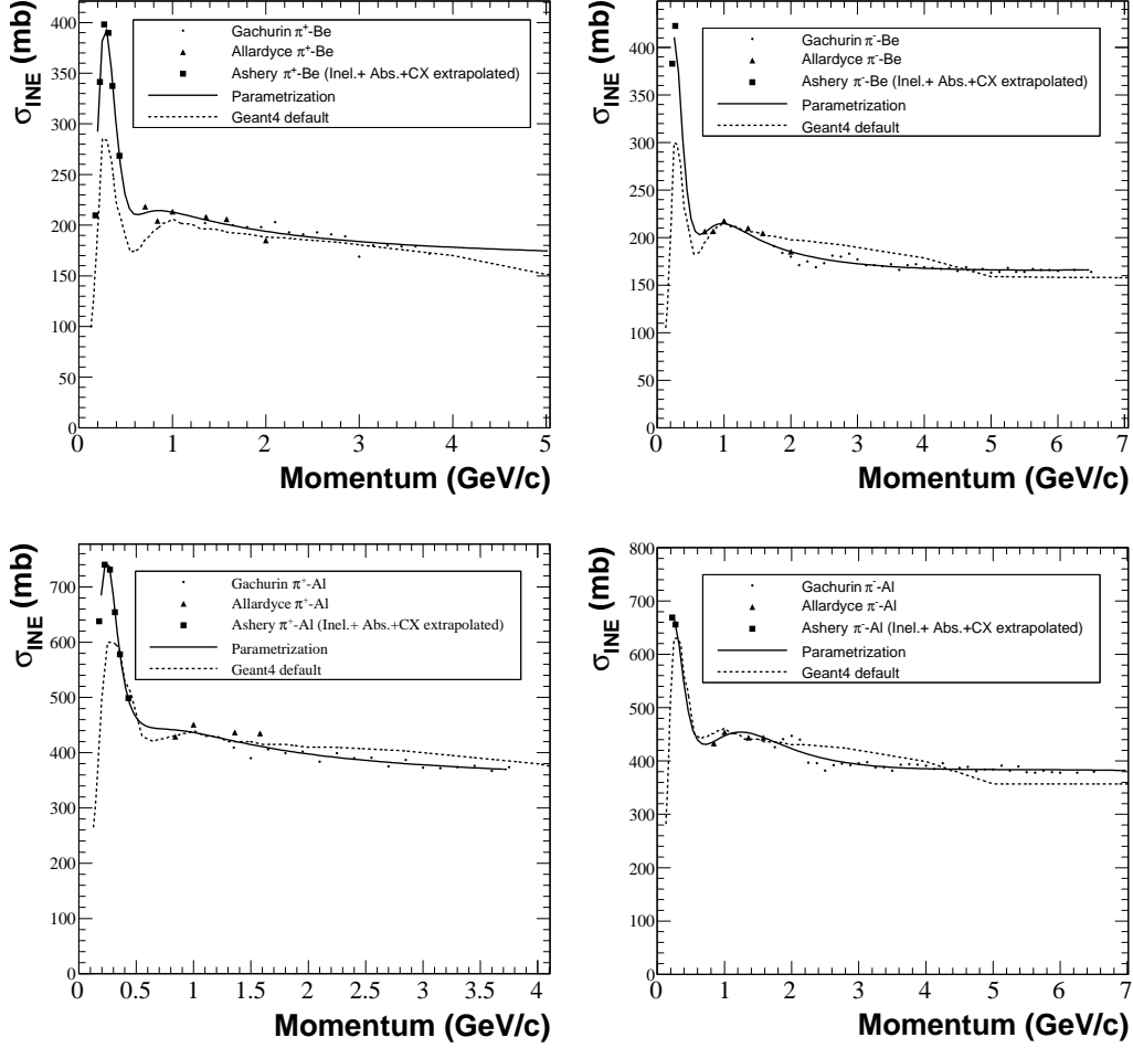
FIG. 15: Inelastic cross sections for \pi^+ -Be (top left), \pi^- -Be (top right), \pi^+ -Al (bottom left) and \pi^- -Al (bottom right) as measured in References [40] (black squares), [41] (black triangles) and [39] (black circles). The solid black lines are the parametrizations used in the flux prediction, while the dashed lines are the default Geant4 parameterizations.
