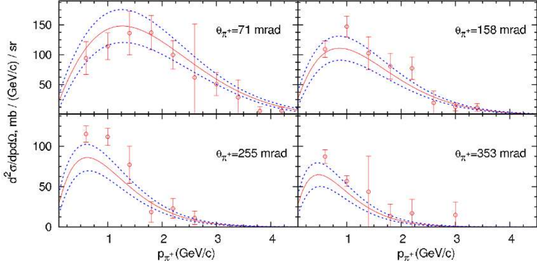
FIG. 20: Comparison of E910 \pi^+ production cross section data [44] (red circles) versus p_\pi in bins of \theta_\pi from 6.4 GeV/c p-Be interactions and best fit SW model (red line). The dashed blue lines represent the uncertainty band for 68% confidence level for 7 fit parameters.
