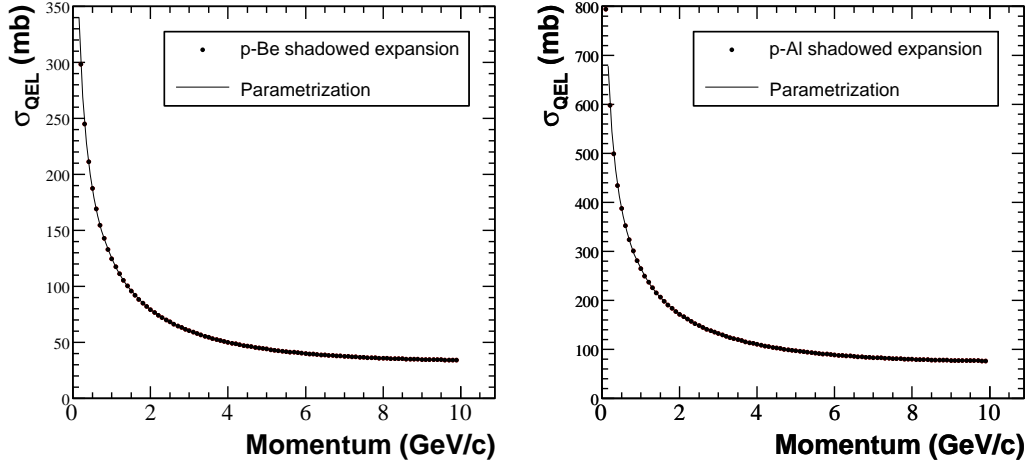
FIG. 16: Calculated values of \sigma_{QEL} for p-Be (left) and p-Al (right) interactions along with the parametrization used in the flux prediction.
