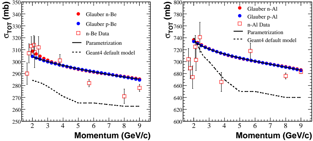
FIG. 11: Total hadronic cross sections calculated using the Glauber model and the optical theorem for beryllium (left) and aluminum (right) targets. The calculated results for neutrons(protons) are shown as red(blue circles). The parameterization used in the flux prediction is shown as the solid black line, while the default Geant4 parameterization is shown as a dashed line. The measured values of \sigma_{TOT} for n-Be/Al from References [32, 33, 34, 35, 36] are shown as red squares.
