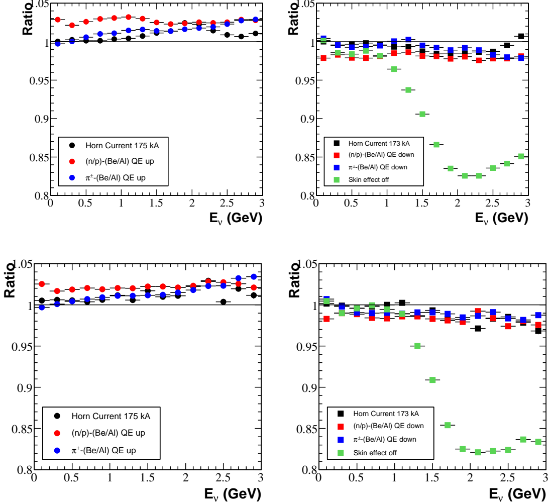
FIG. 40: Top: Change in the \nu_\mu flux from \pi^+ due to the dominant sources of systematic uncertainty apart from particle production. Left: Ratio of flux from increased horn current (black), increased nucleon-nucleus quasi-elastic cross section (red) and increased pion-nucleus quasi-elastic cross section to the default flux. Right: Ratio of flux from decreased horn current (black), decreased nucleon-nucleus quasi-elastic cross section (red), decreased pion-nucleus quasi-elastic cross section (blue), and turning off the skin effect (green), to the default flux. Bottom: Same for predicted \bar{\nu}_\mu flux from \pi^- in antineutrino mode.
