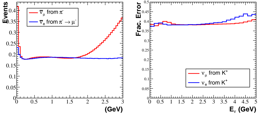
FIG. 34: Left: The fractional uncertainties in the neutrino flux \pi^- \rightarrow \bar{\nu}_\mu and \pi^- \rightarrow \mu^- \rightarrow \bar{\nu}_e flux with the horn in anti-neutrino mode due to uncertainties in the \pi^- production in p-Be interactions. Right: Same for the K^+ \rightarrow \nu_\mu and K^+ \rightarrow \nu_e flux from uncertainties in the K^+ production in p-Be interactions.
