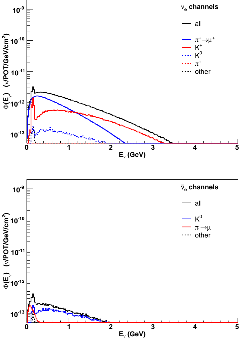
FIG. 30: Predicted \nu_e (top) and \bar{\nu}_e (bottom) flux at the MiniBooNE detector by parent meson species with horn in neutrino mode. The black line is the total predicted flux, while all the subcomponents apart from the dashed black are from nucleon-induced meson production of the indicated decay chains. The dashed black histogram includes all other contributions, primarily from meson decay chains initiated by meson-nucleus interactions.
