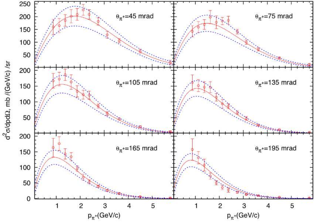
FIG. 19: Comparison of HARP \pi^+ production cross section data [43](red circles) versus p_\pi in bins of \theta_\pi from 8.89 GeV/c p-Be interactions and best fit SW model (red line). The dashed blue lines represent the uncertainty band resulting from varying the parameters within their correlated uncertainties, as described in the text.
