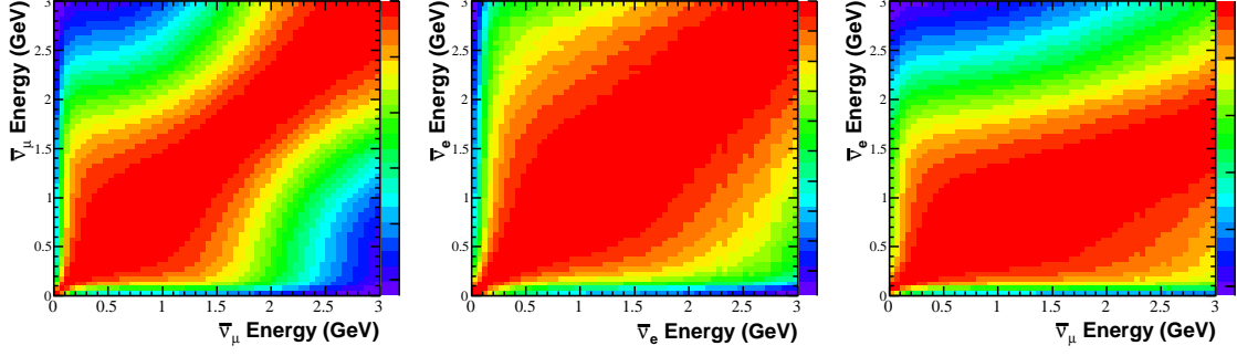
FIG. 37: Left: Correlation matrix for variations in the \pi^- \rightarrow \bar{\nu}_\mu flux due to uncertainties in \pi^- production in p-Be interactions with the horn in anti-neutrino mode. Center/Right: Same for variations in the \pi^- \rightarrow \mu^- \rightarrow \bar{\nu}_e flux (center) and correlations between the \pi^- \rightarrow \bar{\nu}_\mu flux and the \pi^- \rightarrow \mu^- \rightarrow \bar{\nu}_e flux (right). The color scale on each plot ranges from 0 to 1.
