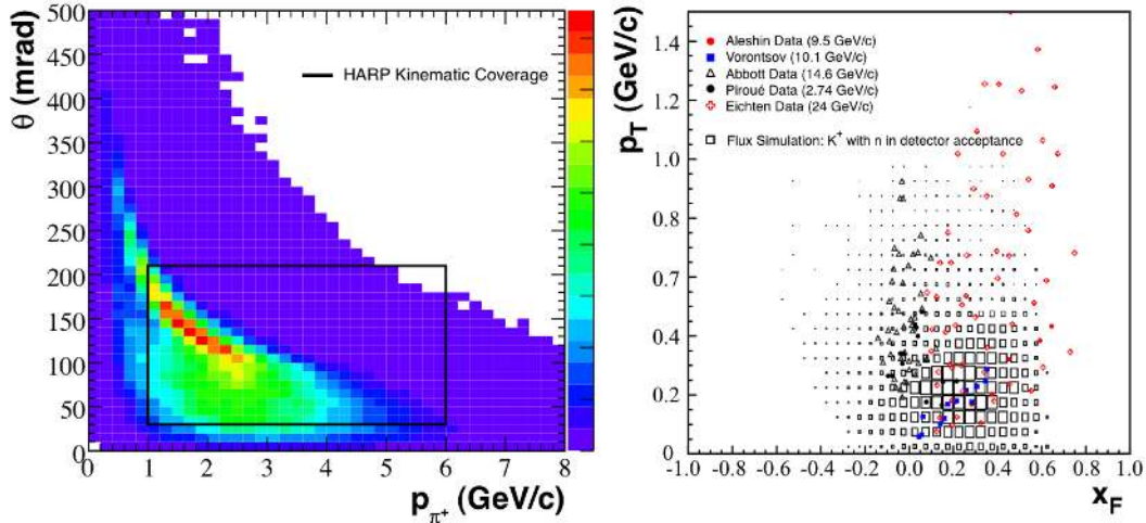
FIG. 18: Left: Production angle vs. \theta vs. momentum p for the \pi^+ in the flux simulation that contribute to the \nu_\mu flux at the MiniBooNE detector. The black box marks the kinematic range covered by the HARP measurements [43]. Right: Transverse momentum p_T vs. the Feynman-scaling variable x_F for the K^+ in the flux simulation that contribute to the neutrino flux at the MiniBooNE detector (black squares). The colored points indicate the kinematic regions measured by p-Be K^+ production measurements [4].
