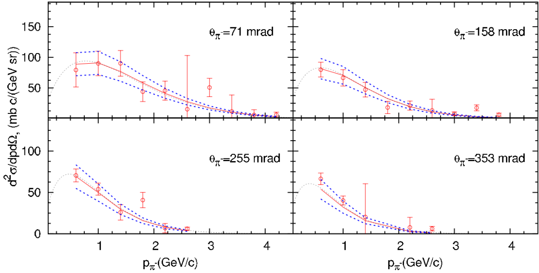
FIG. 23: Comparison of E910 \pi^- production cross section data [44] (red circles) versus p_\pi in bins of \theta_\pi from 6.4 GeV/c p-Be interactions and best-fit SW model (red line). The dashed blue lines represent the uncertainty band resulting from varying the parameters within their correlated uncertainties, as described in the text.
