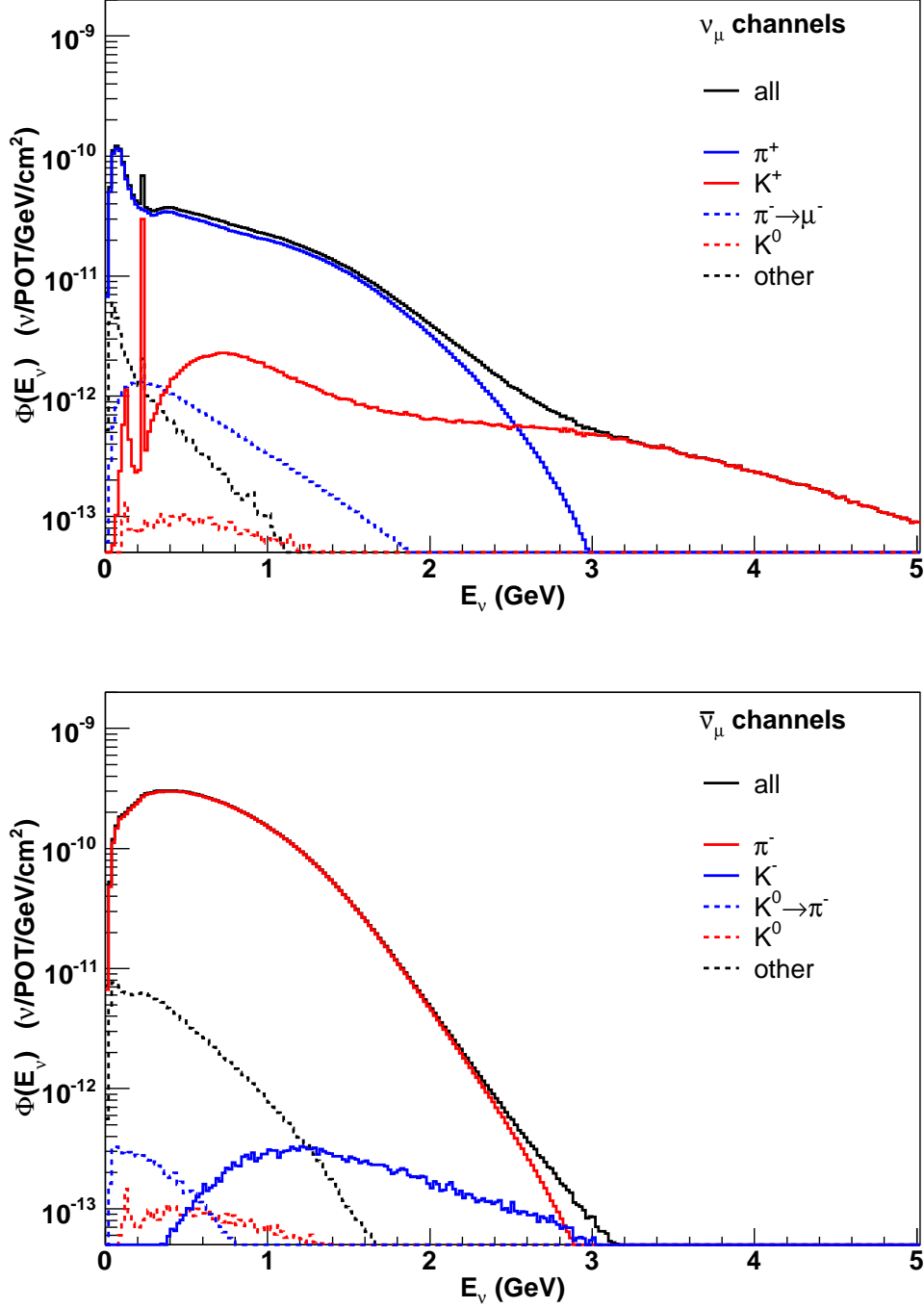
FIG. 31: Predicted \nu_\mu (top) and \bar{\nu}_\mu (bottom) fluxes at the MiniBooNE detector by parent meson species with horn in anti-neutrino mode. The black line is the total predicted flux, while all the subcomponents apart from the dashed black are from nucleon-induced meson production. The dashed black histogram includes all other contributions, primarily from meson decay chains initiated by meson-nucleus interactions.
