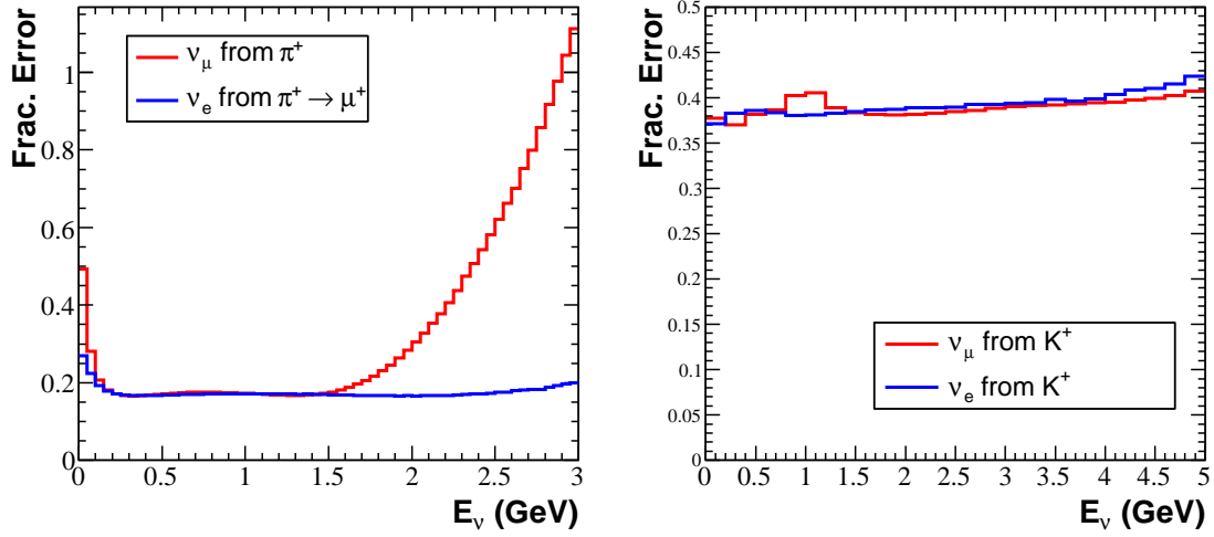
FIG. 33: Left: The fractional uncertainties in the neutrino flux \pi^+ \rightarrow \nu_\mu and \pi^+ \rightarrow \mu^+ \rightarrow \nu_e flux with the horn in neutrino mode due to uncertainties in the \pi^+ production in p-Be interactions. Right: Same for the K^+ \rightarrow \nu_\mu and K^+ \rightarrow \nu_e flux from uncertainties in the K^+ production in p-Be interactions.
