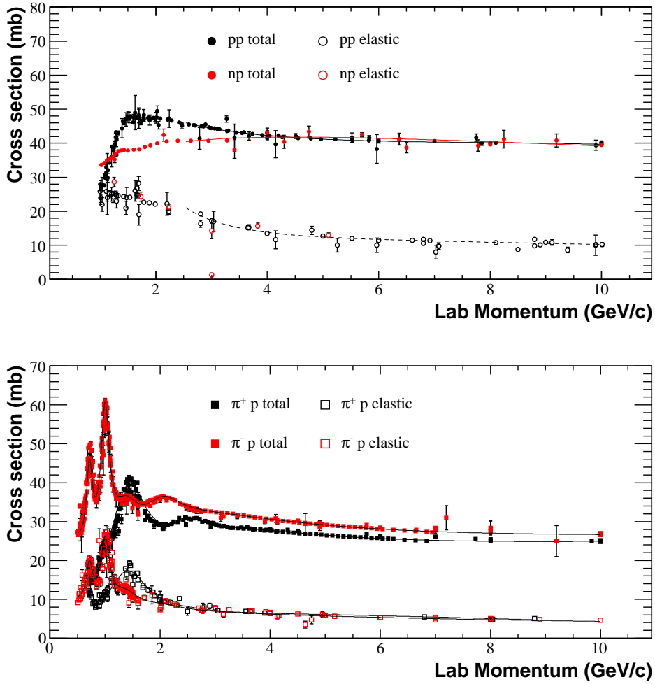
FIG. 7: Total and elastic hadron-proton cross sections (Top: proton/neutron, Bottom: \pi^+/\pi^- ) compiled by the Particle Data Group and Compass [18], with the parametrizations used in the Glauber model calculations.
