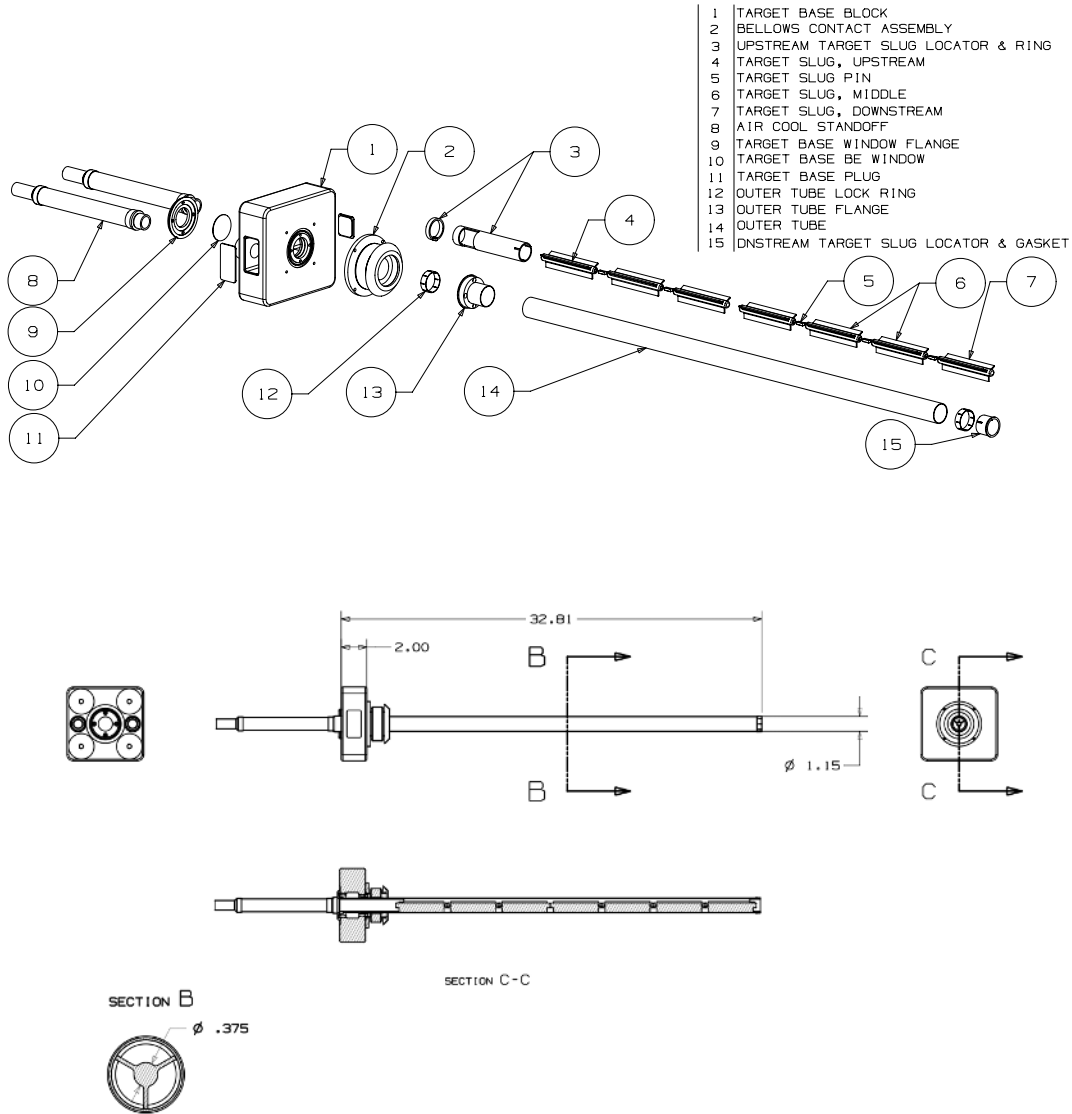
FIG. 2: The MiniBooNE target assembly. The top shows an exploded view of the components, while the bottom shows the assembled configuration. The proton beam enters from the left in both figures, striking the finned beryllium slugs. Dimensions are in inches.
