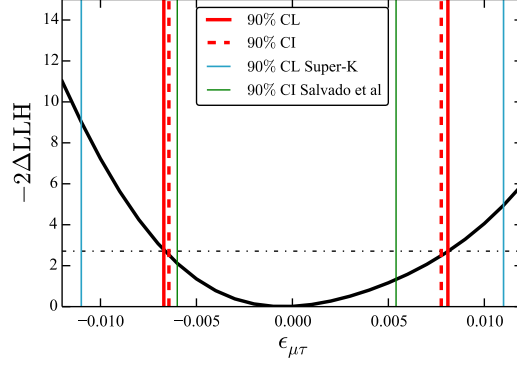
Figure 232: Bound on \varepsilon_{\mu\tau} from different analyses are shown: in blue the analysis by SuperKamiokande, in red the low energy IceCube DeepCore analysis and in green the IceCube high energy NSI bound. Figure from [386]; see also Ref. [384].
