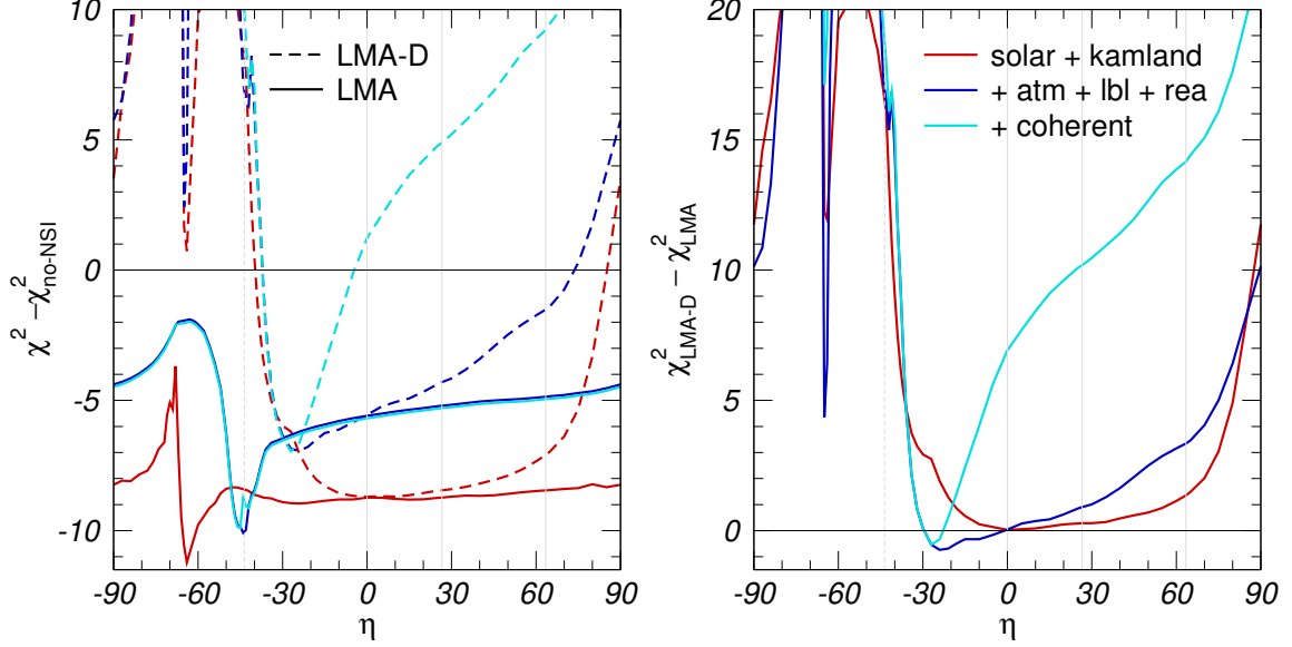
Figure 41: Left: \Delta\chi^2 between the standard ( \chi^2_{\text{no-NSI}} ) and the NSI scenario ( \chi^2(\eta) ) assuming the LMA solution (full lines) or the LMA-D solution (dash lines) for different data combinations as a function of the NSI quark coupling ( \eta ). Right: \Delta\chi^2 between the LMA and LMA-D solutions as a function of \eta .
