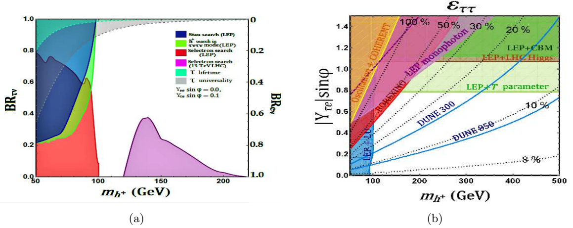
Figure 72: (a) Collider constraints on light charged higgs in the Zee model. (b) \varepsilon_{\tau\tau} prediction. The shaded regions are excluded. See text and Ref. [147] for more details.
