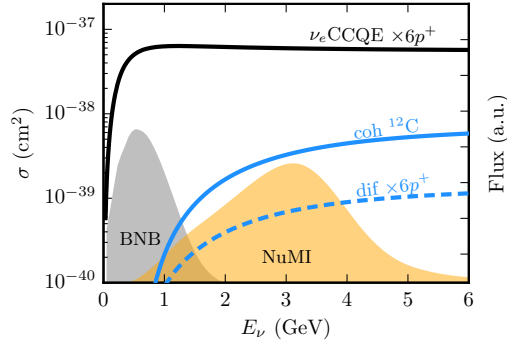
Figure 92: Cross section of dark neutrinos at benchmark point. The benchmark point is the same as in [195]. The blue lines correspond to the dark neutrino production cross section: solid blue for the coherent contribution and dashed blue for the diffractive contribution. For reference the \nu_e charged-current quasielastic cross section is shown as a solid black line.
