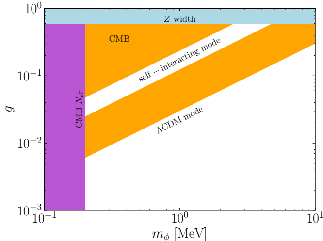
Figure 241: The various constraints on an interaction as described in Eq. (24.1). The new strongly interacting mode is identified by the diagonal white stripe through the orange CMB constrained region.
