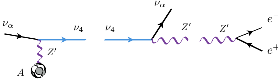
Figure 91: Diagram of production of MiniBooNE signature. A heavy neutrino, \nu_4 , is produced via the exchange of a dark photon with the nucleus. For the realization in [195], m_{Z'} < m_4 and the decay chain follows as shown. In the scenario by [221], m_{Z'} > m_4 and the decay chain shown is forbidden; instead once \nu_4 is produced a three body decay into \nu_\alpha e^+ e^- .
