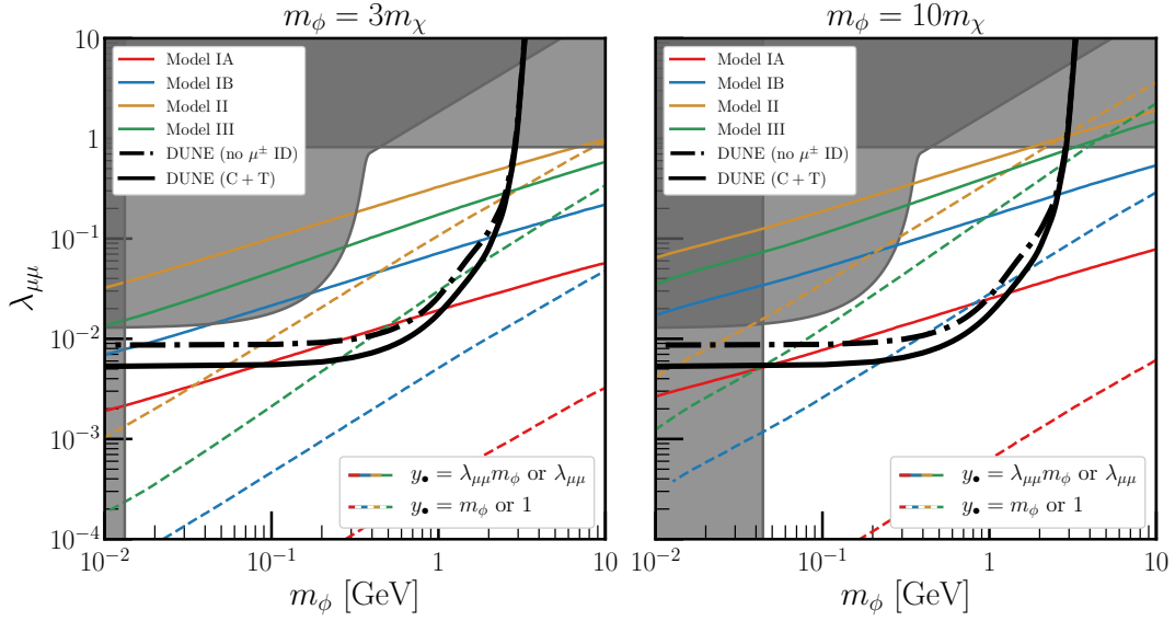
Figure 122: Expected DUNE sensitivity to a scalar \phi with mass m_\phi and coupling to \nu_\mu \lambda_{\mu\mu} assuming 10 years of data collection at the near detector. Solid black line: sensitivity using charge-identification techniques, Dot-dashed black line: no charge identification. Colored lines indicate thermal relic targets for the dark matter scenarios discussed in the text.
