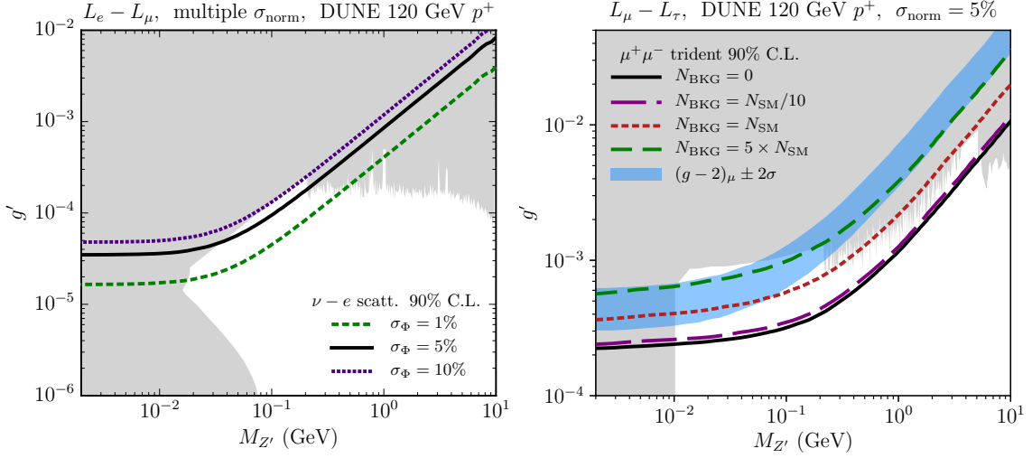
Figure 182: The DUNE ND sensitivity to L_e - L_\mu (left) and L_\mu - L_\tau (right) model with no kinetic mixing at 90% C.L. On the left panel we vary the normalization uncertainty from a pessimistic 10% to an aggressive 1% value, and on the right we vary the background to dimuon tridents from 0 to a total of 5 times the number of SM dimuon events after cuts.
