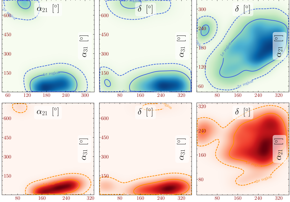
Figure 101: The two-dimensional projections for intermediate scale leptogenesis with M_1 = 3.16 \times 10^6 GeV for x_1 = 0 , y_2 = 0 , x_3 = 180^\circ , y_1 = y_2 = 180^\circ , with CP violation provided only by the phases of the PMNS matrix. The normal ordered case is colored blue/green and inverted ordering orange/red and contours correspond to 68% and 95% confidence levels. We fix m_1 = 0.21 eV, the mixing angles of the PMNS matrix and mass squared splittings of the light neutrinos are fixed at their best fit values as given by global fit data [245]. This plot was created using SUPERPLOT [246].
