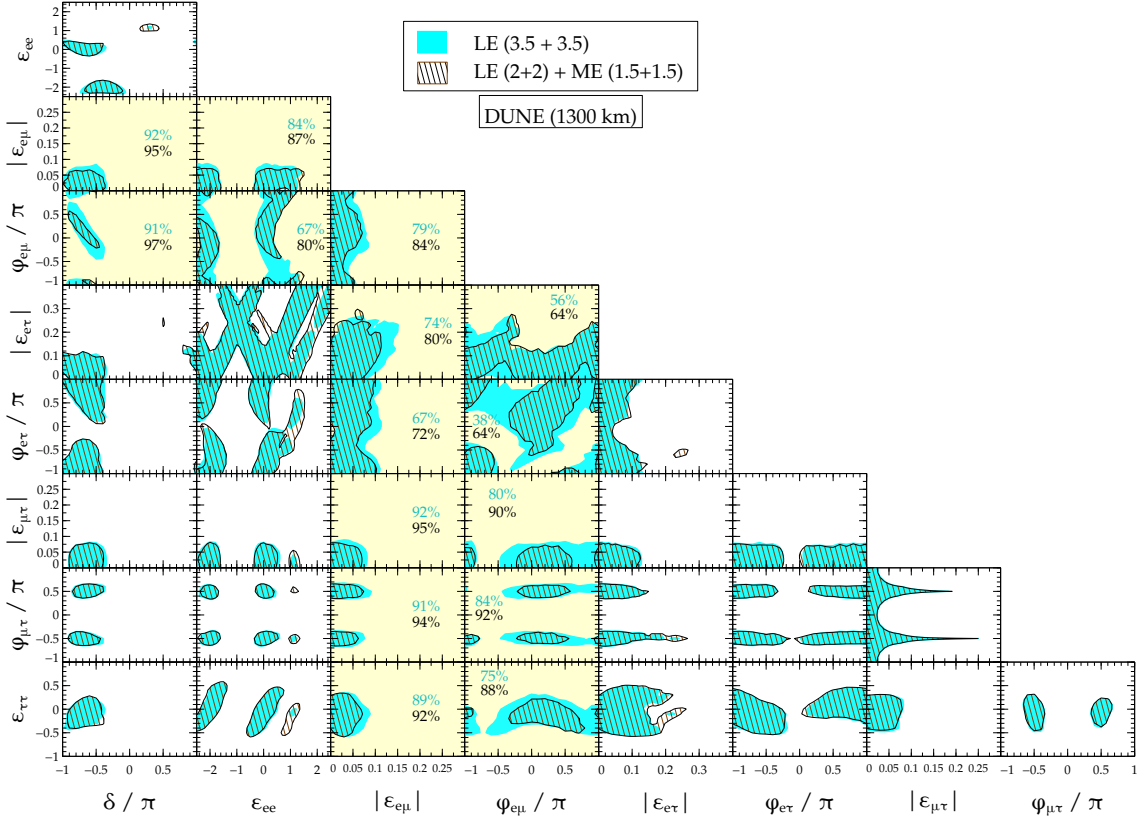
Figure 225: A comparison of the sensitivity of DUNE to probe the NSI parameters at 99% confidence level when a standard low energy (LE) beam tune is used (cyan region) and when a combination of low and medium energy (LE + ME) beam tune is used (black hatched region), keeping the total runtime same (3.5 years of \nu + 3.5 years of \bar{\nu} run) for both scenario. In the latter case, the total runtime is distributed between the LE beam (2 years of \nu + 2 years of \bar{\nu} ) and the medium energy beam (1.5 years of \nu + 1.5 years of \bar{\nu} ). The panels with a light yellow (white) background indicate significant improvement (no improvement) by using LE + ME beam over using LE only. The numbers in the light yellow shaded panels correspond to the area lying outside the contour for the two cases (cyan for LE and black for LE+ME) expressed as a percentage of the total parameter space plotted. These numbers quantify the improvement over the LE only option when the ME beam tune is used in conjunction with the LE beam tune in these panels. (taken from [382])
