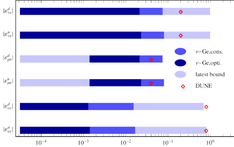
Figure 171: Future coherent bounds on NSIs, from Ref. [269].
