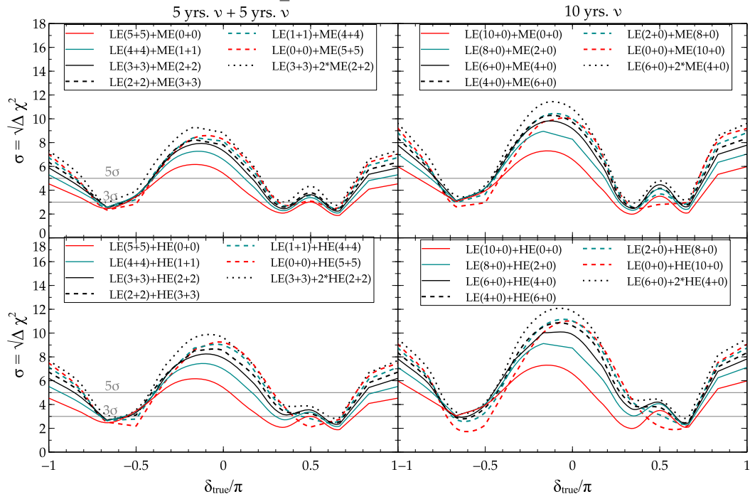
Figure 223: Separation between SI and NSI events at DUNE with different beam tunes at \chi^2 level. A CP conserving NSI scenario is assumed. The left column shows 5 years of neutrino and 5 years of anti-neutrino run times, while the right column depicts the case of 10 years of neutrino run time only. The plot is taken from [370].
