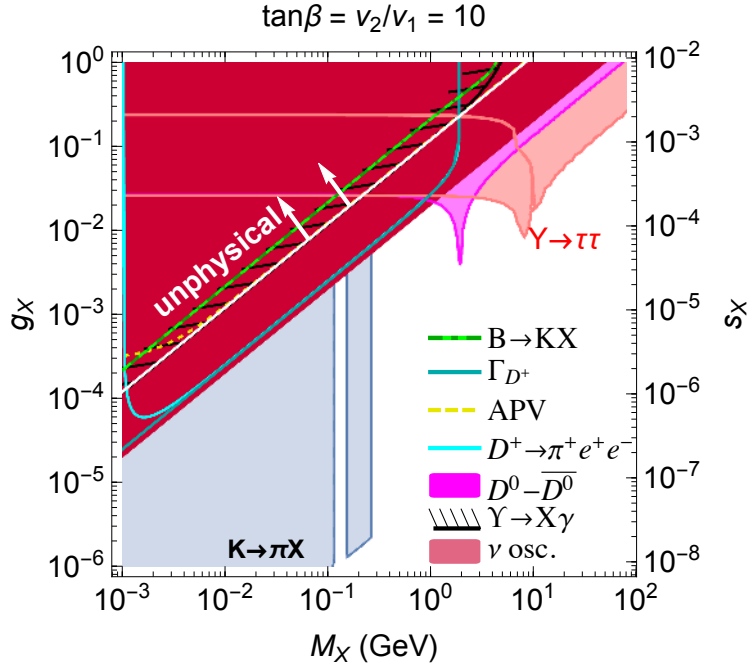
Figure 151: Constraints on the U(1)_{B-L}^{(3)} gauge boson mass M_X and coupling g_X for \tan\beta = 10 . For convenience the X - Z mixing, s_X , is also shown. Notice that for a given g_X , the mass of the gauge boson M_X is bounded from below, so there is an unphysical region in the upper left corner of the M_X \times g_X plane (delineated by the white line). The “ \nu osc.” bound comes from non standard interaction effects (matter potential) on atmospheric neutrinos. “APV” refers to atomic parity violation. Here the charged Higgs mass, relevant to the B \rightarrow KX constraint, is taken to be 1200 GeV.
