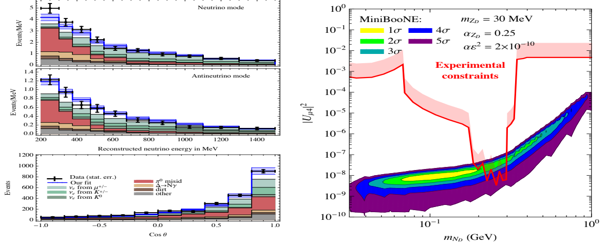
Figure 82: Left: The MiniBooNE electron-like event data [169] in the neutrino (top panel) and antineutrino (middle panel) modes as a function of E_\nu^{\text{rec}} , as well as the \cos \theta distribution (bottom panel) for the neutrino data. Note that the data points have only statistical uncertainties, while the systematic uncertainties from the background are encoded in the light blue band.. The predictions of our benchmark point m_{N_D} = 420 MeV, m_{Z_D} = 30 MeV, |U_{\mu 4}|^2 = 9 \times 10^{-7} , \alpha_D = 0.25 and \alpha \varepsilon^2 = 2 \times 10^{-10} are also shown as the blue lines. Right: Region of our model in the |U_{\mu 4}|^2 versus m_{N_D} plane satisfying MiniBooNE data at 1\sigma to 5\sigma CL, for the hypothesis m_{Z_D} = 30 MeV, \alpha_D = 0.25 and \alpha \varepsilon^2 = 2 \times 10^{-10} . The region above the red curve is excluded at 99% CL by meson decays, the muon decay Michel spectrum and lepton universality [108, 170].
