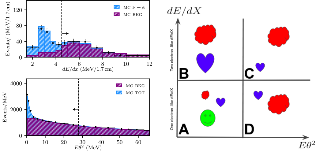
Figure 93: Data plots used in the analysis and a cartoon that explains how they are related. Left top: Distribution of Minerva low-energy mode neutrino-electron cross section event selection without the dE/dx cut. We use the rate of events to the right of the cut, as signalled by the arrow, to place perform our analysis. Left bottom: Distribution of CHARM-II neutrino-electron cross section analysis without the E\theta^2 cut. The rate to the left of the cut, as pointed by the arrow, is used in our analysis. Right: The content of the different parts of phase space in the two variables used in our analysis, dE/dx and E\theta^2 . The Minerva distribution used in our analysis corresponds to panels A and B, while the CHARM-ii information used corresponds to panels A and D. The markers signal electron-neutrino (green happy face), di-electrons produced in the dark neutrino model (purple heart), and backgrounds such as neutral-current \pi_0 (red clouds). The sizes of the markers are meant to illustrate their relative contributions, though exact sizes are experiment and dark neutrino parameter-point dependent; the location of the makers within each of the panels (A,B,C, and D) does not have meaning.
