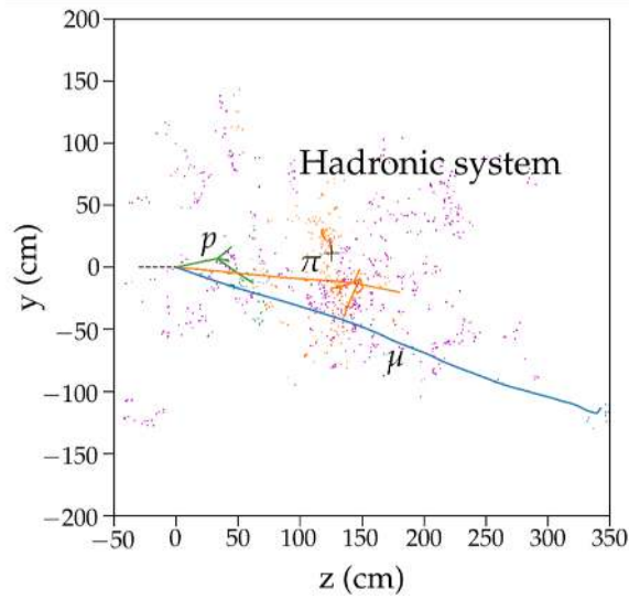
Figure 211: An example simulated 4 GeV \nu_\mu event using GENIE and FLUKA. The magenta energy deposits are caused by neutrons undergoing multiple scatterings; the orange color denotes energy originally carried by the prompt charged pion. The figure is taken from Ref. [368].
