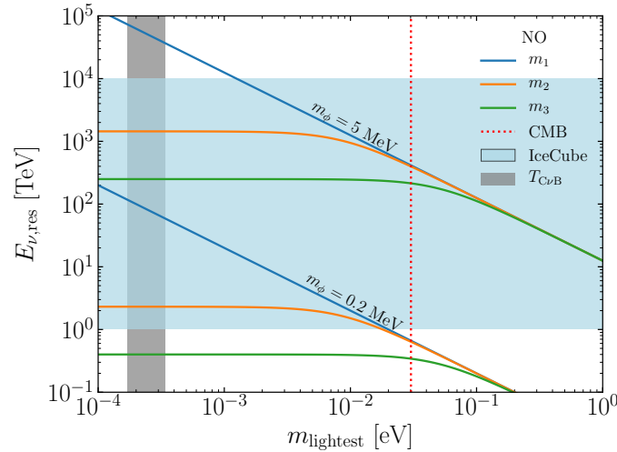
Figure 242: The resonant energy of each of the three C\nu B mass eigenstates as a function of the lightest neutrino mass in the normal mass ordering. The blue band is the broadest range of energies that IceCube could possibly measure the astrophysical neutrino flux. The red dashed line indicates the limit from cosmology [262].
