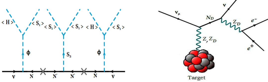
Figure 81: Left: diagram for the dynamically induced light neutrino masses in our model; Right: contributions to the cross section that in our model gives rise to MiniBooNE’s excess of electron-like events.
