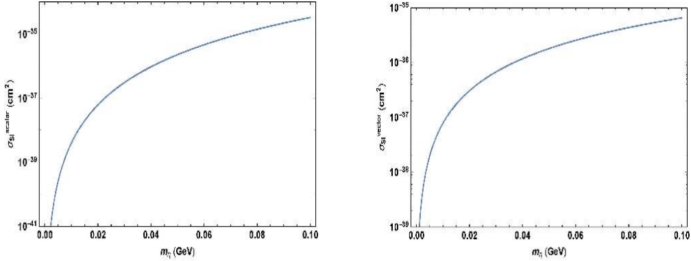
Figure 132: Dark matter-nucleon scattering cross section as a function of the dark matter mass. The cross sections are calculated for m_\phi = 100 MeV, \delta = 0 and V = 10 GeV. These dark matter-nucleon cross sections are allowed by CRESST III, XENON1T and CDEX-1B constraints.
