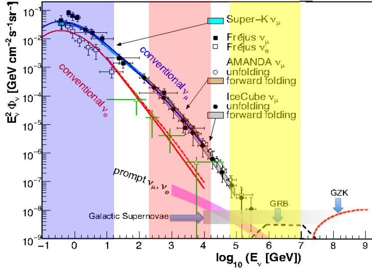
Figure 231: Atmospheric neutrino flux, with data from different experiments, the first two shaded regions (blue, red) show the approximate range of real neutrino energy for the low and high energy data samples used to perform oscillation analysis by IceCube. The energy range of the measured astrophysical neutrinos is shown in yellow.
