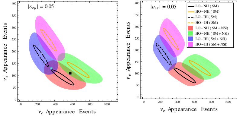
Figure 191: Figure represents the bi-event plot for DUNE setup. In case of SM ellipses, the running parameter is \delta , whereas in case of SM+NSI blobs, the running parameters are \delta and \phi_{e\mu} ( \delta and \phi_{e\tau} ) in the left (right) panel respectively. For details please see the text and [31]. This figure has been taken from [31].
