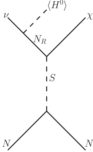
Figure 172: A process to produce dark matter in CEVNS proposed in Ref. [271].
