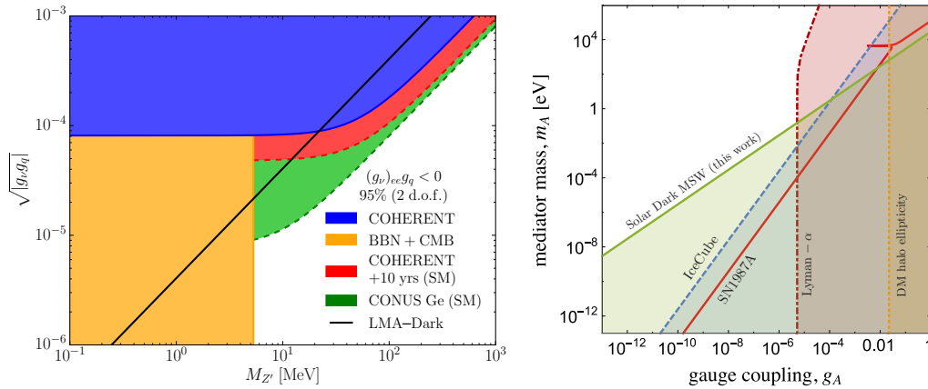
Figure 141: Light mediator NSI ( left panel ) is still large enough to account for LMA-Dark, but only in a narrow range of masses [20]. Large matter effects ( right panel ) can come about in models of dark matter-neutrino interactions [290].
