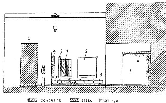
FIG. 8. Detector assembly of the neutrino experiments I–III at Gösigen. The central detector, normally located within the concrete house H is shown in its rolled out position. (1) is the central detector unit, (2) are the tanks of the active veto, (4) are water tanks, (5) is a movable concrete closing door. The various parts of the detector move on a system of rails (3).
