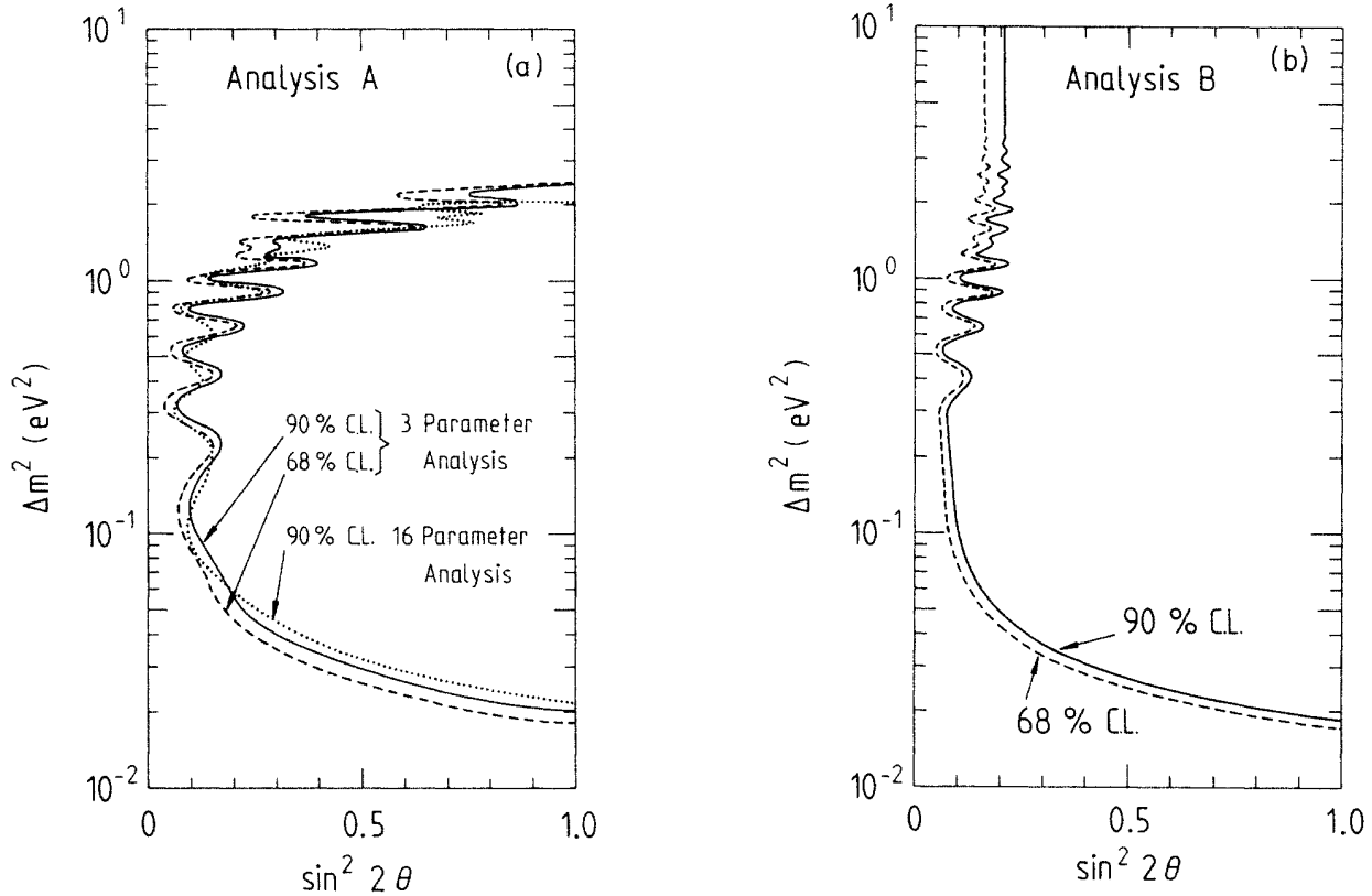
FIG. 13. (a) Exclusion plot for the oscillation parameters \Delta m^2 and \sin^2 2\theta , relying exclusively on the information obtained in experiments I–III. The solid (90% C.L.) and dashed (68% C.L.) curves represent confidence contours of an analysis which relies on the reactor antineutrino spectrum S_A(E_\nu) obtained from the best common fit to experiments I–III. The dotted curves give the 90% C.L. for another analysis which uses independent parameters for each energy bin to characterize a positron spectrum (Sec. VI C). The areas to the right of the curves are excluded. The result is consistent with the absence of neutrino oscillations. (b) Exclusion plot for the oscillation parameters \Delta m^2 and \sin^2 2\theta , combining the results of experiments I–III with measured detector efficiencies, the reaction cross section (neutron half-life 622 sec) and the reactor antineutrino spectrum as derived from independent \beta -spectrum measurements. The result is consistent with the absence of neutrino oscillations.
