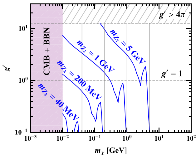
Fig. 11 Values of the DM mass m_\chi and the coupling g' required to reproduce the observed relic abundance. We have fixed m_{Z_2} = 0.04, 0.2, 1, and 5 GeV, and have considered the representative case of \theta_e = 0.031 , while keeping \theta_{\mu,\tau} = 0 . Along (above) the blue lines the DM relic density matches (is less than) the observed value. We do not consider m_\chi > m_{Z_2} to ensure the neutrino portal regime. The lower bound m_\chi \gtrsim 10 MeV is set by observations of the CMB and BBN
