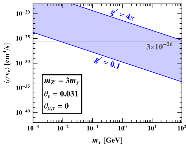
Fig. 7 Thermally averaged annihilation cross section multiplied by the relative velocity for \chi\bar{\chi} \rightarrow \nu\bar{\nu} . We have fixed m_{Z'} = 3m_\chi, \theta_e = 0.031, \theta_\mu = \theta_\tau = 0, and varied g' between 0.1 and 4\pi
