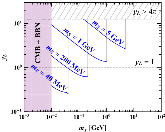
Fig. 6 Values of the DM mass m_\chi and the coupling y_L required to reproduce the observed relic abundance. We have fixed m_S = 0.04, 0.2, 1, and 5 GeV, and have considered the representative case of \theta_e = 0.031 , while keeping \theta_{\mu,\tau} = 0 . Along (above) the blue lines the DM relic density matches (is less than) the observed value. The lower bound m_\chi \gtrsim 10 MeV is set by observations of the CMB and BBN
