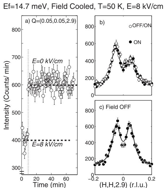
FIG. 5. Panel (a) plots the diffuse scattering intensity at \vec{Q}=(0.05,0.05,2.9) as a function of time. The electric field was abruptly turned off and the leads electrically shorted to ground at the time indicated by the dashed line. Panels (b) and (c) show examples of linear scans of the diffuse scattering before and after the field is turned off. The open circles in panel (b) show the diffuse scattering measured with the field turned back on \sim 70 min after the field was turned off. The diffuse scattering reproduces the field-cooled intensity.
