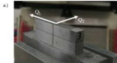
Figure 2a) and b). Pictures of samples C and A, respectively, as mounted on SMARTS. The white arrows in a.) represent the longitudinal (L) and transverse (T) diffraction vectors defined by the instrument geometry. The tear between the substructure and the growth plate is indicated by the white arrow.
