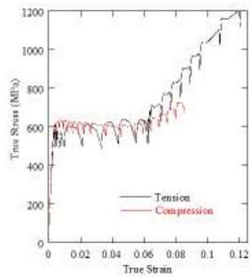
Figure 3. Stress-strain curves of as-deposited GP-1 in tension and compression.
