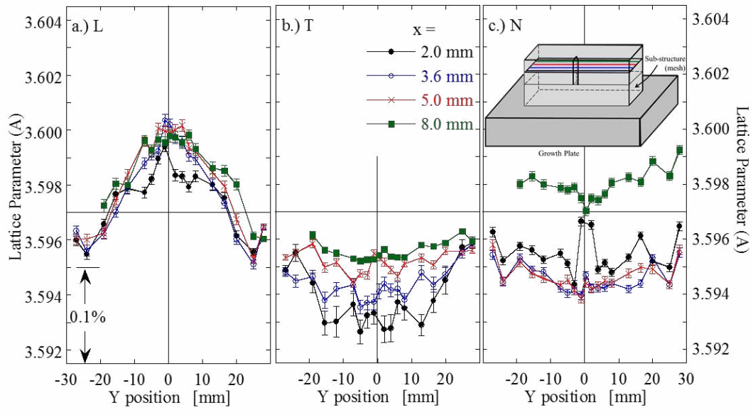
Figure 4a-c. Longitudinal (y) line profiles of L, T, and N-direction lattice parameters on an x-y plane (at z = 5.0mm) at increasing values of x in Specimen C. The inset schematic in c.) highlights the locus of measurement points (colors matched to plots) on the specimen.
