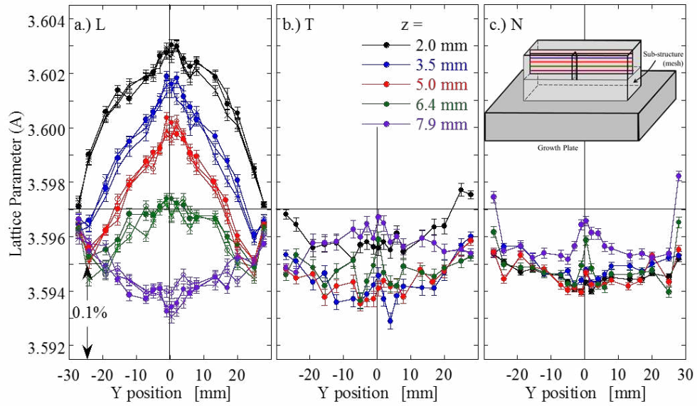
Figure 5a-c. Longitudinal (y) line profiles of L, T, and N-direction lattice parameters on a y-z plane (at x = 3.8 mm) at increasing values of z. z = 10 mm is at the interface with the mesh sub-structure and z = 0 mm is the free surface. a.) includes data from samples C (solid circles), D (open circles) and K (x's). b. and c.) only include data from sample C. The inset schematic in c.) highlights the locus of measurement points (colors matched to plots) on the specimen.
