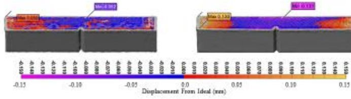
Figure 7a and b. Displacement of top surface of Charpy specimen M from ideal defined by the CAD drawing before and after removal from the base plate and substructure.
